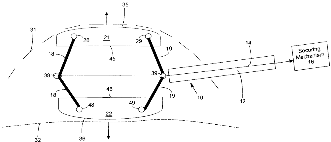
DEPLOYED CONFIGURATION
