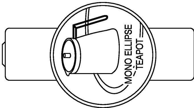
OBJECT RECOGNITION
