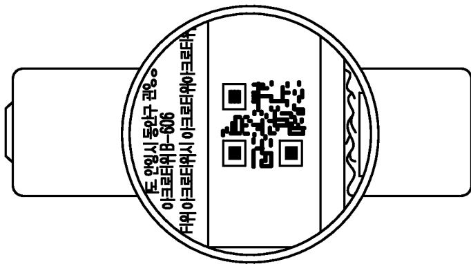
BARCODE RECOGNITION
