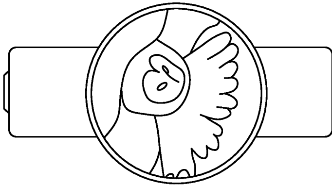
IMAGE RECOGNITION
