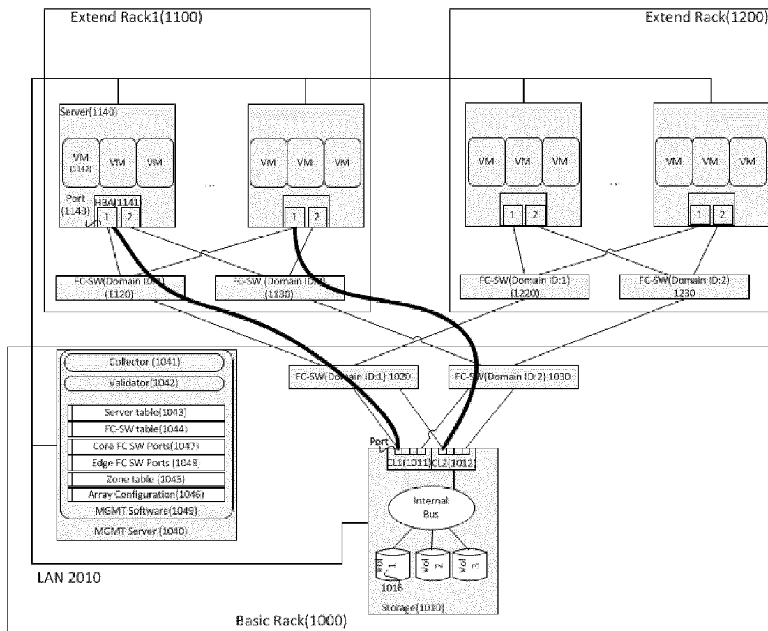
Fig 2 Logical Configuration
