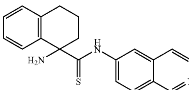
1-amino-N-(isoquinolin-6-yl)-1,2,3,4-tetrahydronaphthalene-1-carbothioamide
