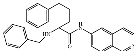
2-(benzylamino)-N-(isoquinolin-7-yl)-5-phenylpentanamide
