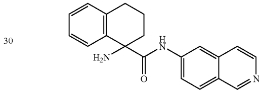
1-amino-N-(isoquinolin-6-yl)-1,2,3,4-tetrahydronaphthalene-1-carboxamide
