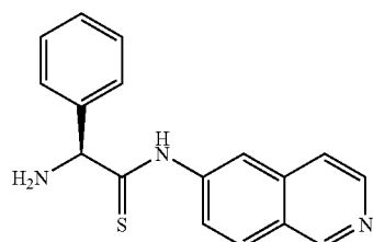
(S)-2-amino-N-(isoquinolin-6-yl)-2-phenylethanethioamide
