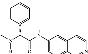
(R)-N-(isoquinolin-6-yl)-2-(methylamino)-2-phenylacetamide
