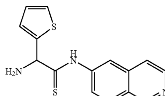
2-amino-N-(isoquinolin-6-yl)-2-(thiophen-2-yl)ethanethioamide
