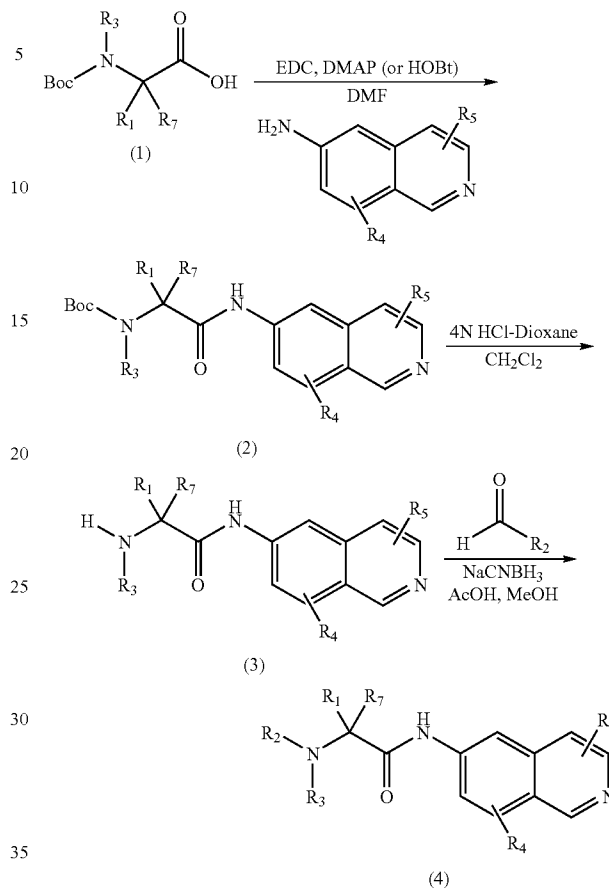
Scheme One
