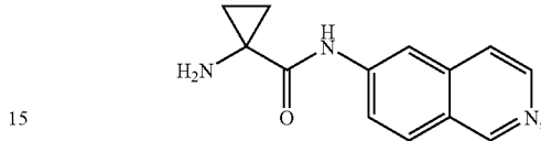
1-amino-N-(isoquinolin-6-yl)cyclopropanecarboxamide
