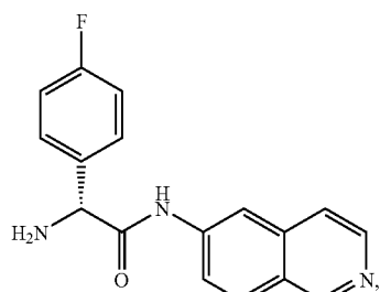
(R)-2-amino-2-(4-fluorophenyl)-N-(isoquinolin-6-yl)acetamide
