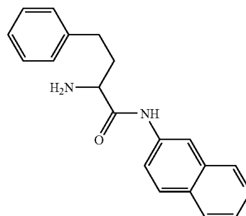
2-amino-N-(isoquinolin-7-yl)-4-phenylbutanamide
