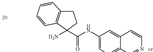
1-amino-N-(isoquinolin-6-yl)-2,3-dihydro-1H-indene-1-carboxamide
