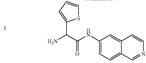
2-amino-N-(isoquinolin-6-yl)-2-(thiophen-2-yl)acetamide
