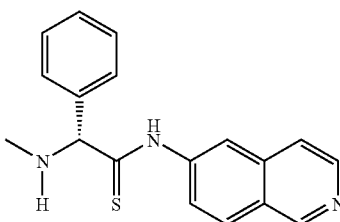
(R)-N-(isoquinolin-6-yl)-2-(methylamino)-2-phenylethanethioamide
