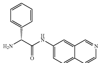
(R)-2-amino-N-(isoquinolin-7-yl)-2-phenylacetamide
