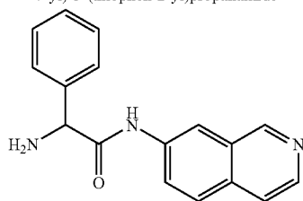
2-amino-N-(isoquinolin-7-yl)-2-phenylacetamide
