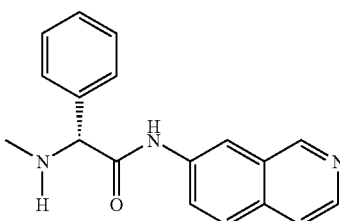
(R)-N-(isoquinolin-7-yl)-2-(methylamino)-2-phenylacetamide
