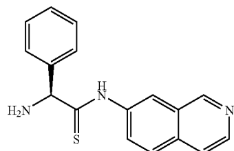
(S)-2-amino-N-(isoquinolin-7-yl)-2-phenylethanethioamide
