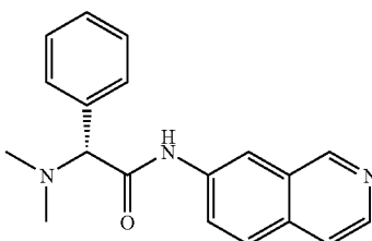
(R)-2-(dimethylamino)-N-(isoquinolin-7-yl)-2-phenylacetamide
