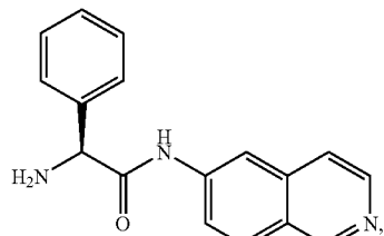
(S)-2-amino-N-(isoquinolin-6-yl)-2-phenylacetamide
