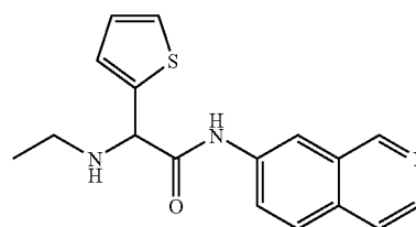
2-(ethylamino)-N-(isoquinolin-7-yl)-2-(thiophen-2-yl)acetamide
