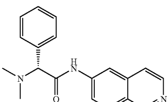
(R)-2-(dimethylamino)-N-(isoquinolin-6-yl)-2-phenylacetamide
