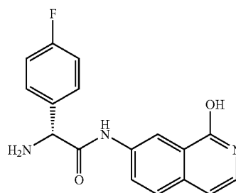
(R)-2-amino-2-(4-fluorophenyl)-N-(1-hydroxyisoquinolin-7-yl)acetamide
