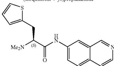
(S)-2-(dimethylamino)-N-(isoquinolin-7-yl)-3-(thiophen-2-yl)propanamide
