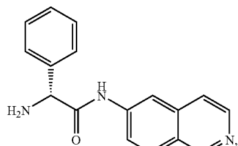
(R)-2-amino-N-(isoquinolin-6-yl)-2-phenylacetamide
