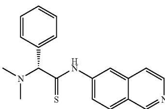
(R)-2-(dimethylamino)-N-(isoquinolin-6-yl)-2-phenylethanethioamide
