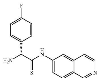
(R)-2-amino-2-(4-fluorophenyl)-N-(isoquinolin-6-yl)ethanethioamide
