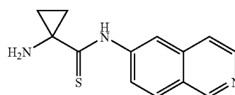
1-amino-N-(isoquinolin-6-yl)cyclopropanecarbothioamide
