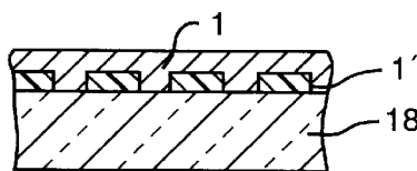
FIG. 6B (PRIOR ART)
