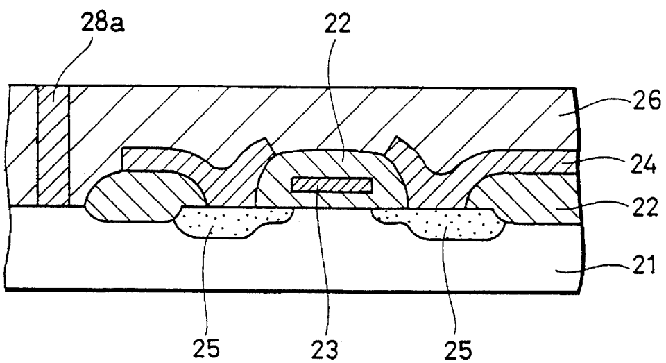
FIG. 23 PRIOR ART
