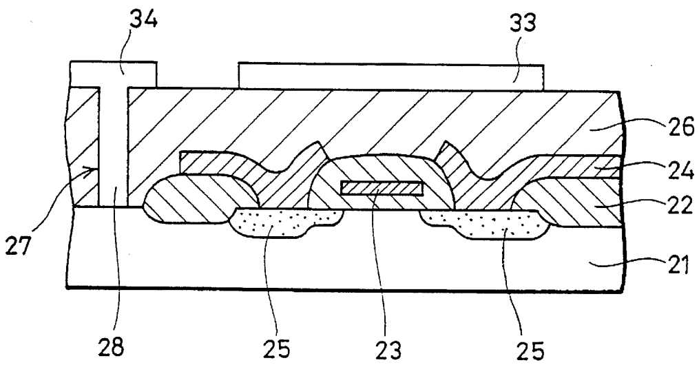
FIG. 25 PRIOR ART
