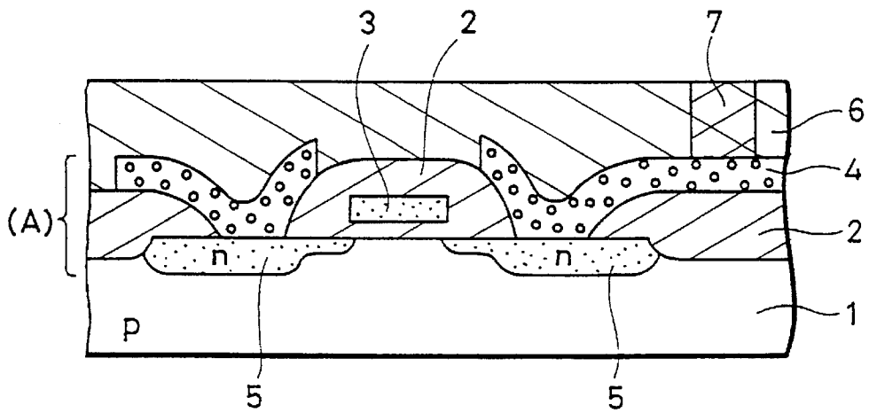
FIG.19 PRIOR ART
