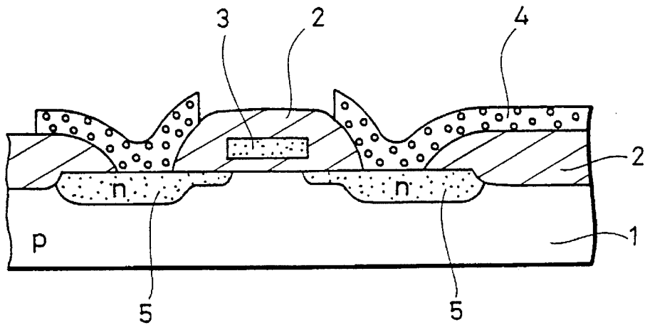
FIG.17 PRIOR ART
