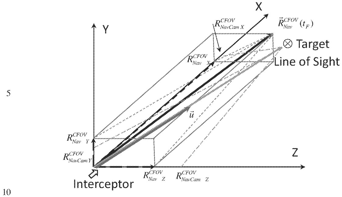
Figure 6 : Illustration of relative position in CFOV frame
