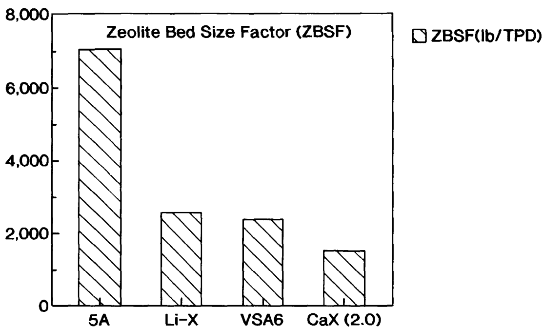
A Graphic Comparison of the Quantity of CaX(2.0), 5A, LiX and VSA6 Zeolite Adsorbents in the Illustrated Four Bed PSA Process.
