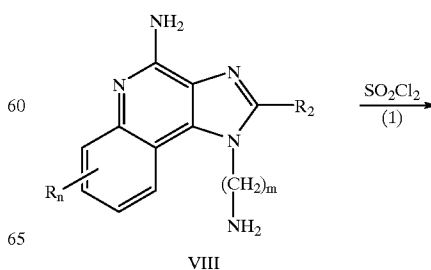
Reaction Scheme V
