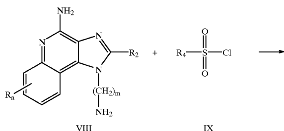
Reaction Scheme II
