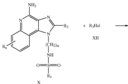
Reaction Scheme IV
