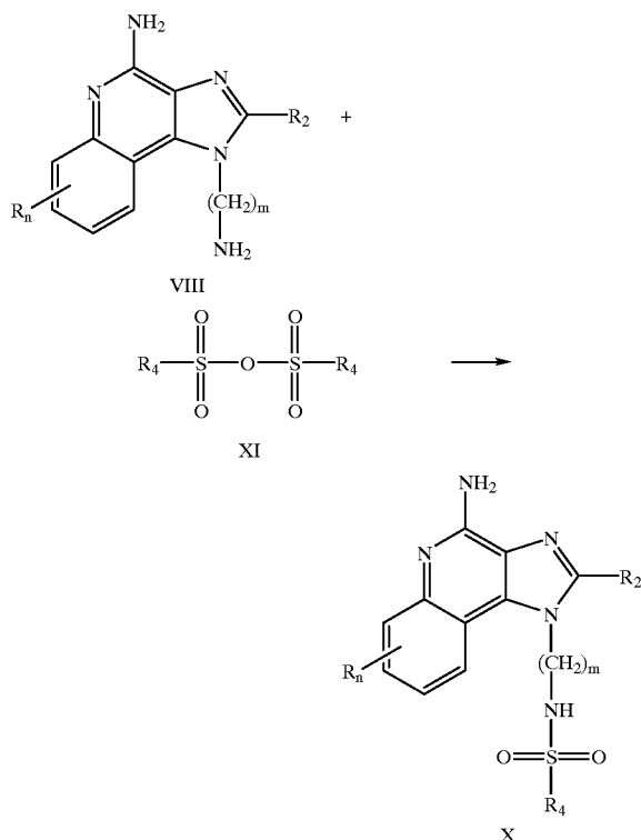
Reaction Scheme III
