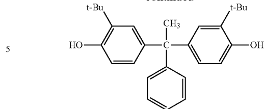
BisOTBP-AP
