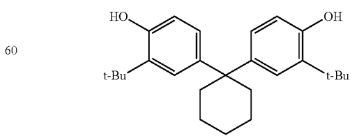
BisOTBP-Z
