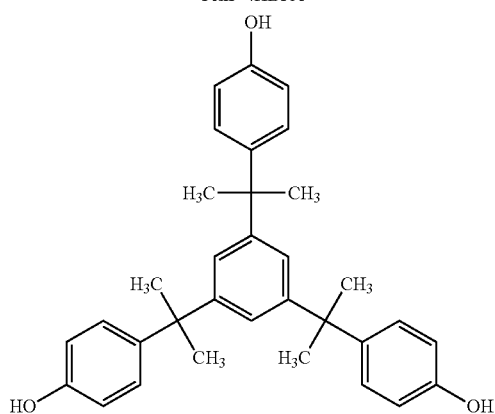
TrisP-TC
