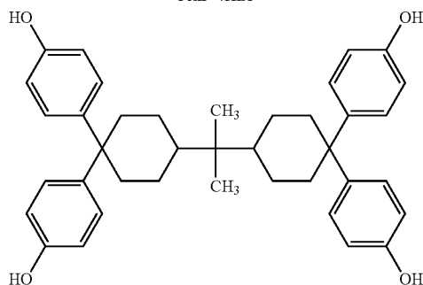
TekP-4HBPA
