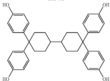
TekP-4HBP
