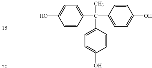
TrisP-HAP
