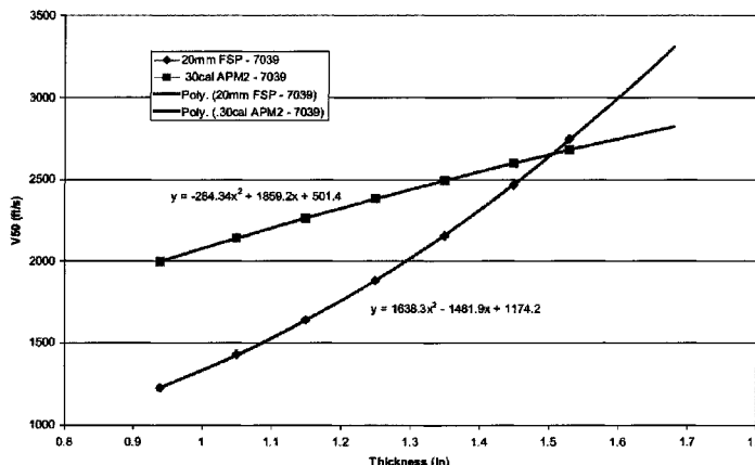
V50 vs. Thickness for 7039
