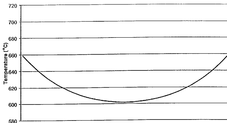
Reactant exit temperature profile across heat exchanger
