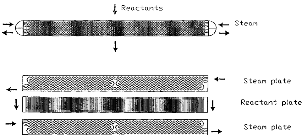
FIGURE 8: “Ported” style of plate construction.
