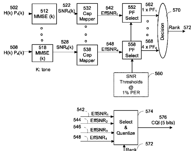
Performance Based Rank Prediction
