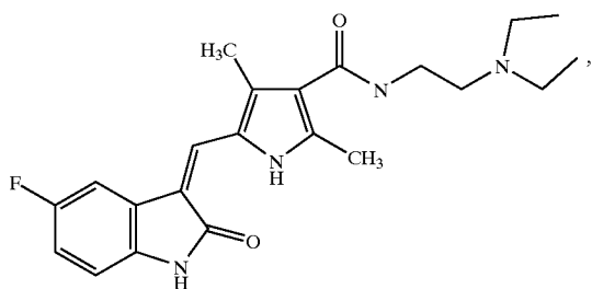
Compound 2
