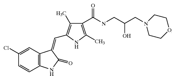
Compound 7
