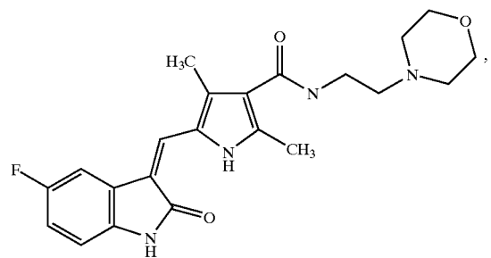
Compound 3
