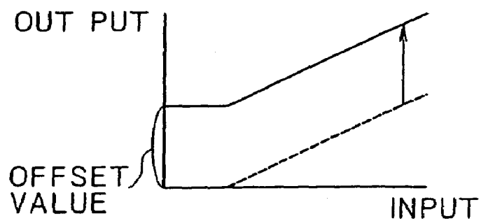
INPUT/OUTPUT CHARACTERISTIC
