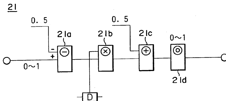
CONSTITUTION OF EMPHASIS/DEEMPHASIS CIRCUIT
