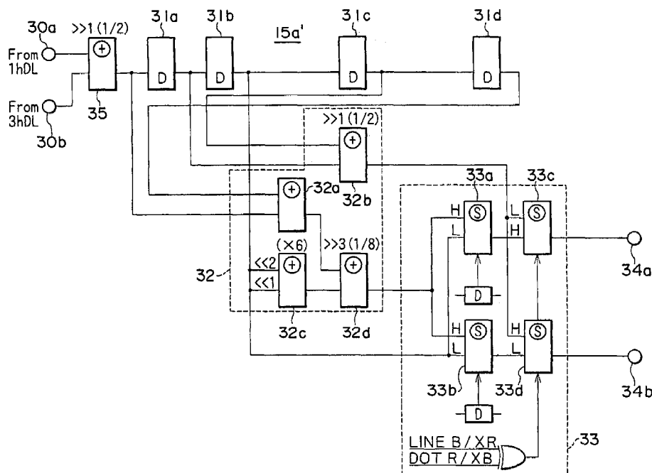
CONSTITUTION OF HORIZONTAL-DIRECTION INTERPOLATOR
