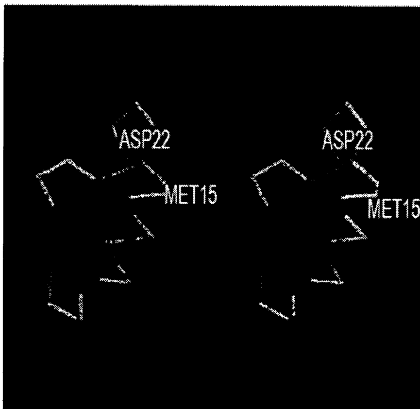
AZURIN TRUNCATION WITH ALPHA-HELICAL STRUCTURE
