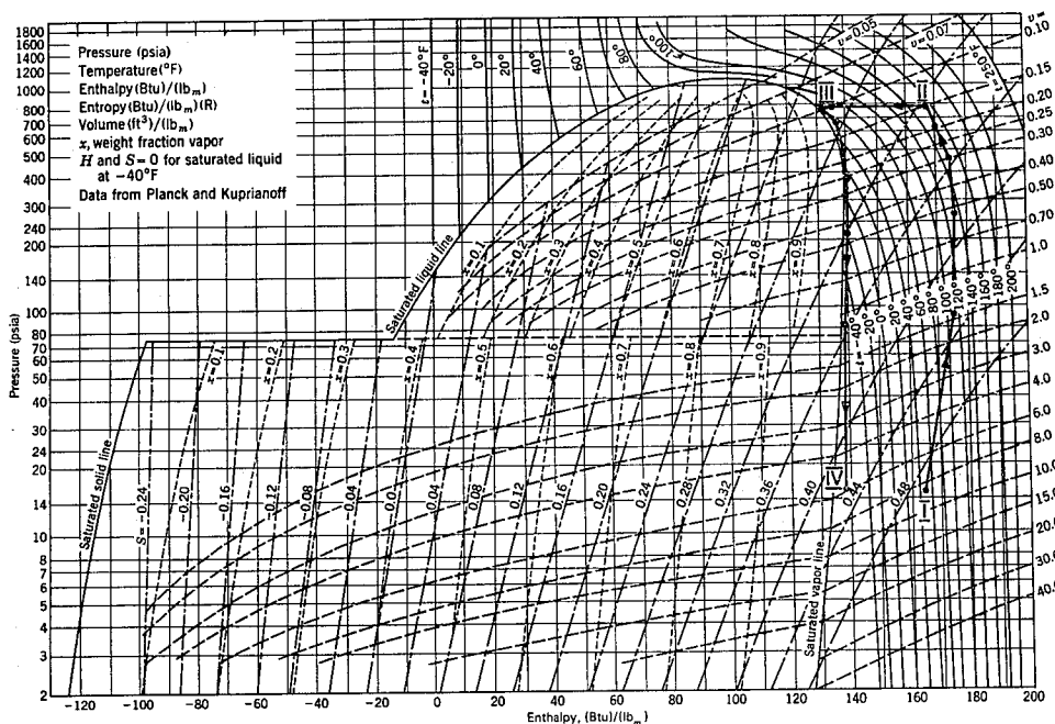
Pressure-enthalpy diagram for carbon dioxide.
