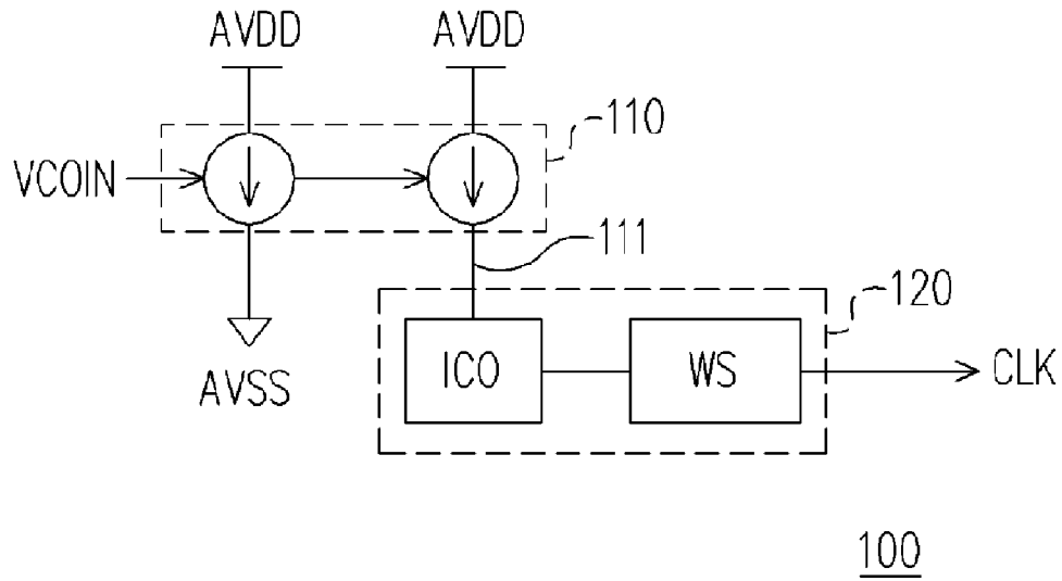
FIG. 1A(PRIOR ART)
