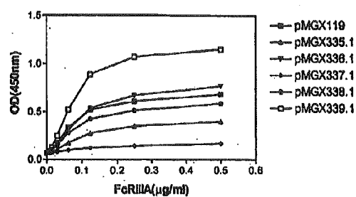
B. 3G8 binds to FcRIIA-G2 and mutants
