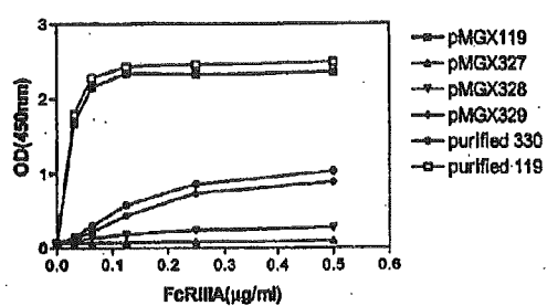
A. 3G8 binds to FcRIIA-G2 and mutants
