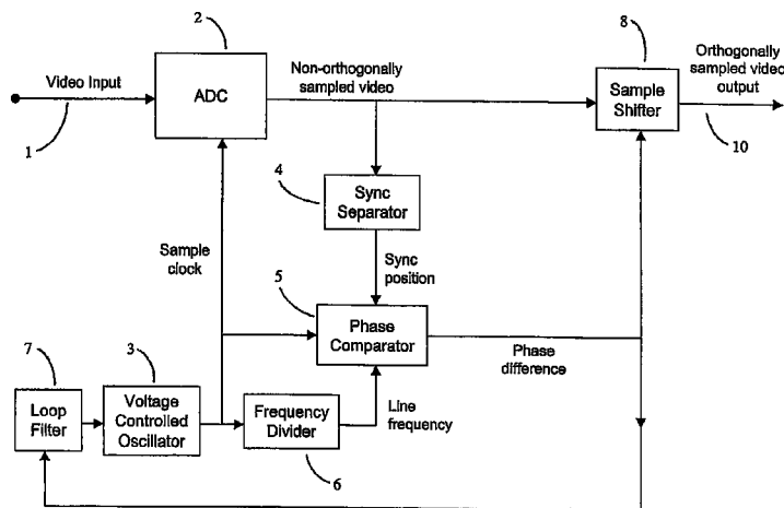
Video ADC System
