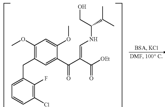
Compound 8a C 26 H 31 ClFNO 6 Mol. Wt.: 507.98
