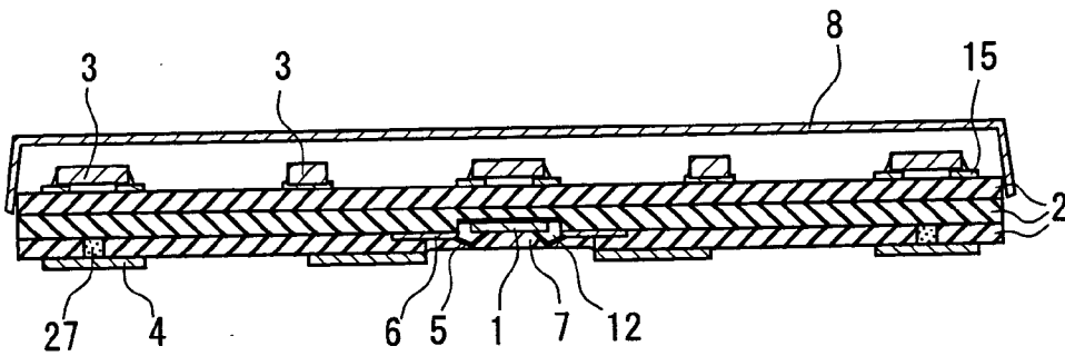
FIG. 11 PRIOR ART
