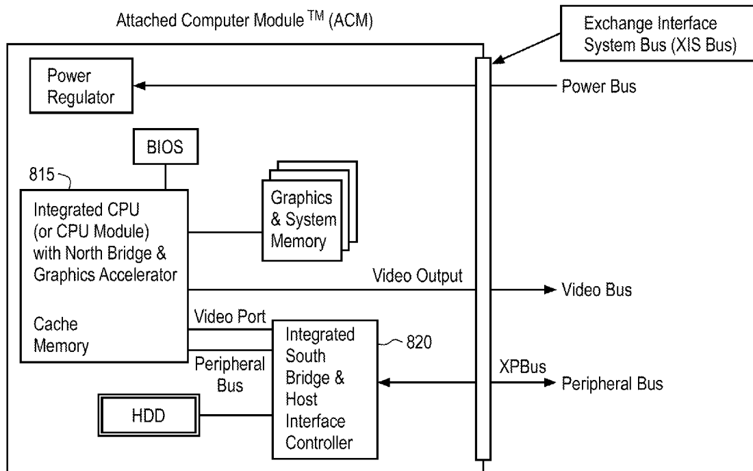
Attached Computer Module with Integrated CPU/NB/Graphics and Integrated HIC/SB
