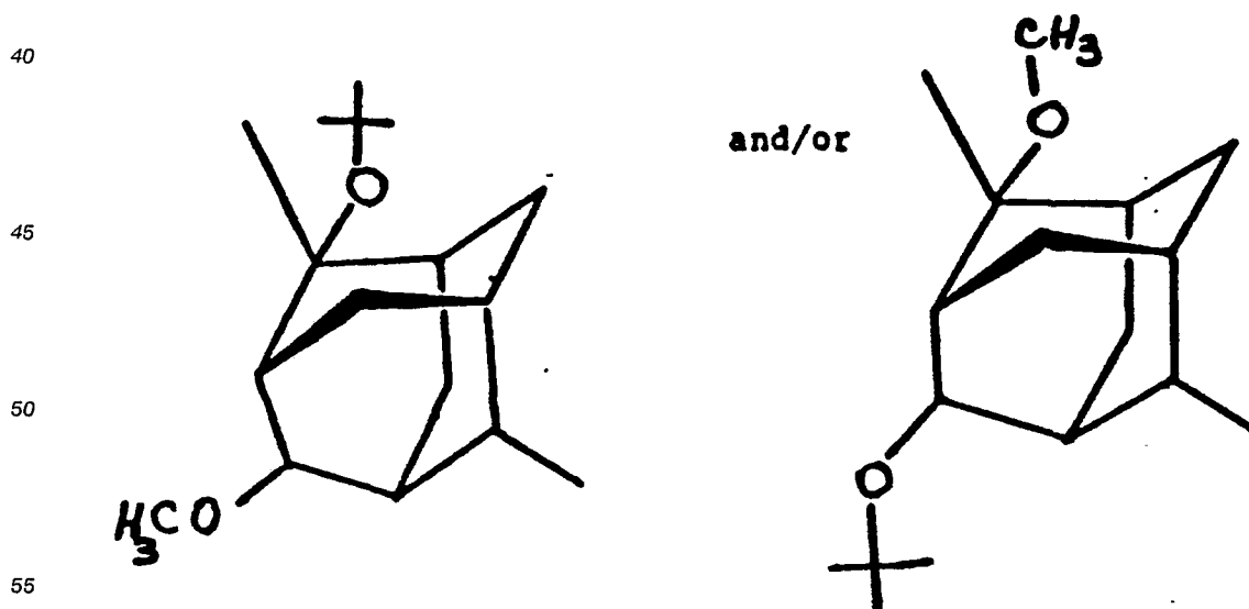
Figure 41 is the NMR spectrum for the peak group 393 of the GLC profile of Figure 39 of the
