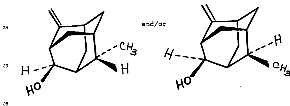
Figure 45 is the GLC profile for the crude reaction product of Example XVI containing the compound having the structure:
