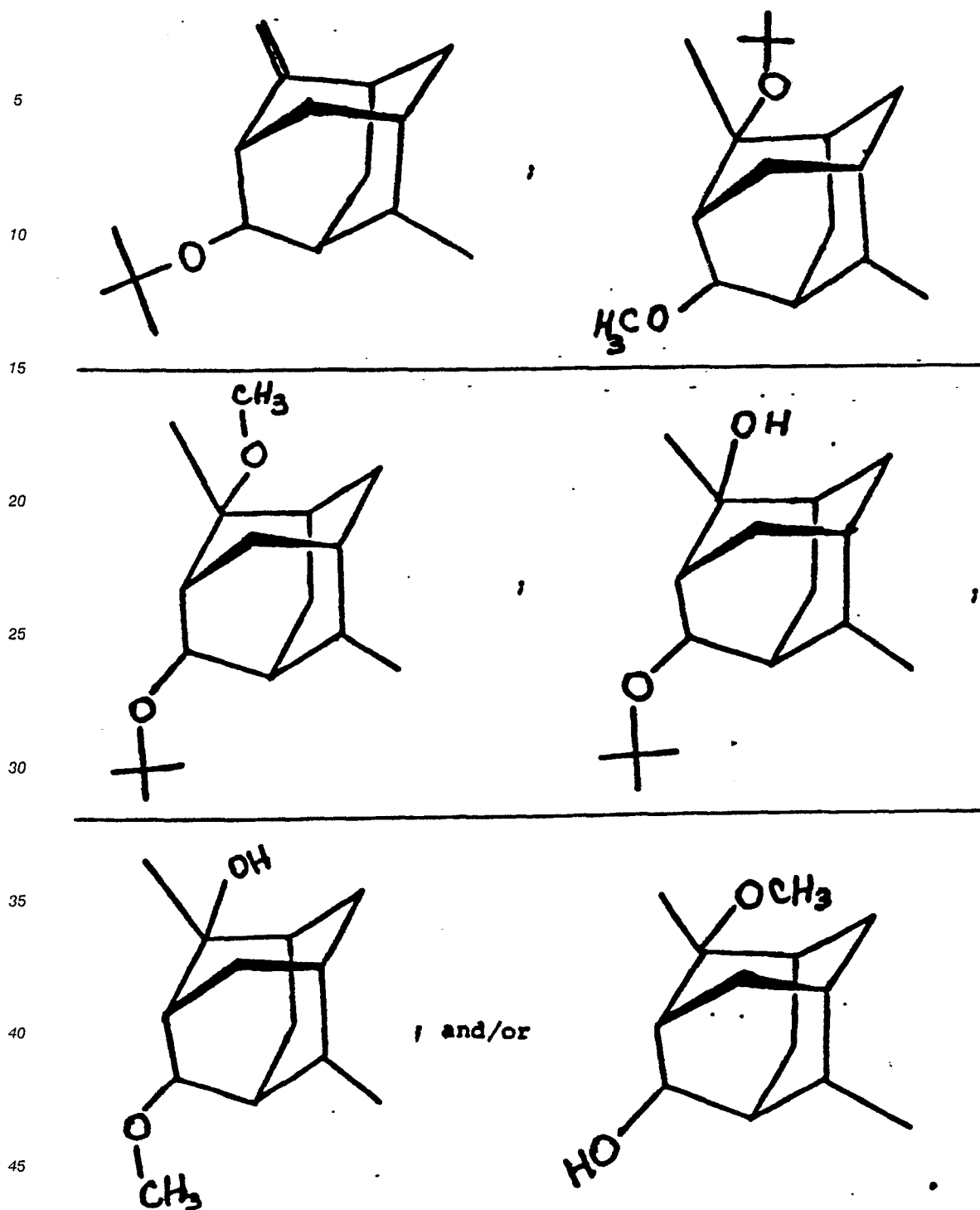
Figure 37B is the GLC profile for distillation fraction 3 of the distillation product of the reaction product of Example XV containing the compounds having the structures:
