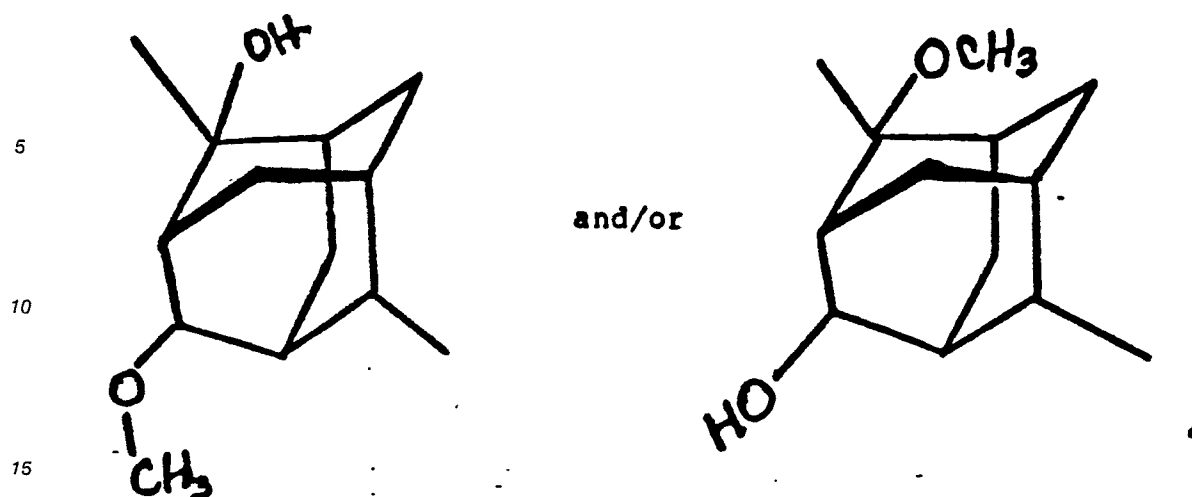
Figure 44 is the NMR spectrum for the peak indicated by reference numeral 372 of the GLC profile of Figure 37C; and is for one or both of the epimers having the structures:
