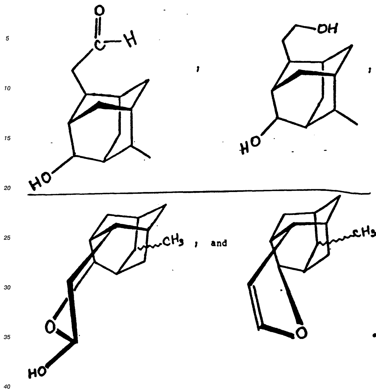
Figure 37A is the GLC profile for the crude reaction product of Example XV containing the compounds having the structures:
