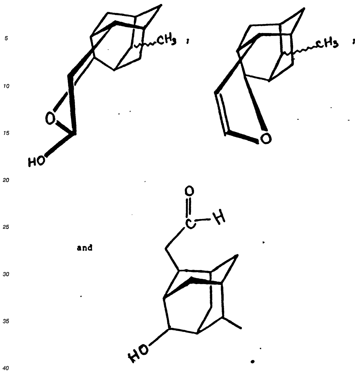
Figure 37 is the NMR spectrum for distillation fraction 8 of the distillation product of the reaction product of Example XIV containing the compounds having the structures:
