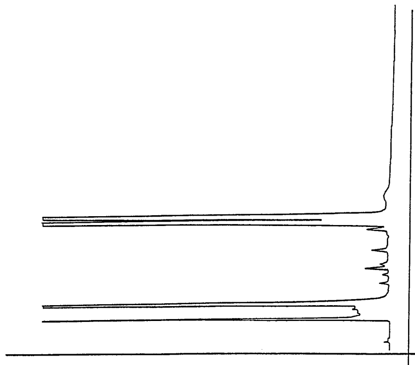
GLC PROFILE FOR EXAMPLE VI.
