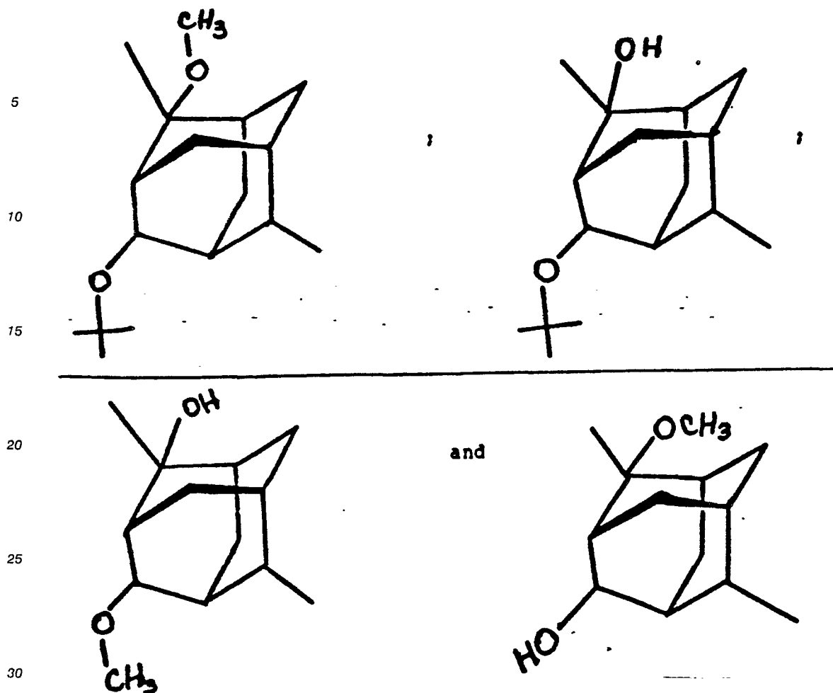
Figure 40 is the NMR spectrum for peak group 392 of the GLC profile of Figure 39 for distillation fraction 6 of the distillation product of the reaction product of Example XV; one or a mixture of the compounds having the structures:
