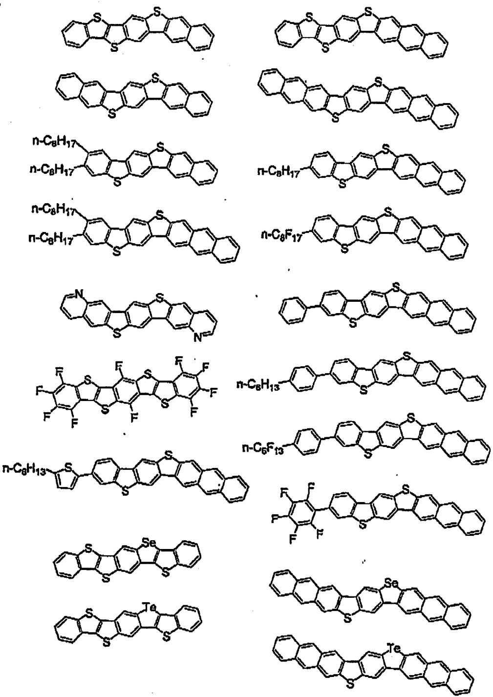
[Chem 13]
