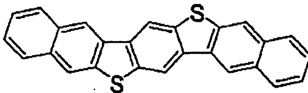
[Chem 32]
