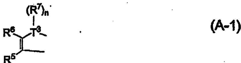
[Chem 10]
