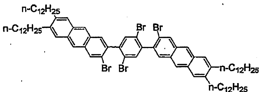
[Chem 33]
