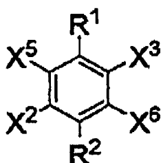
[Chem 19]
