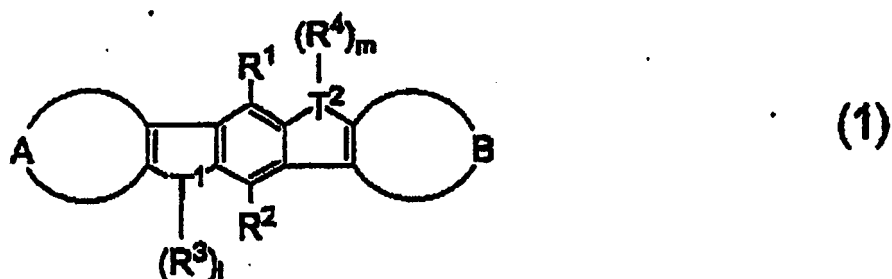
[Chem 1]
