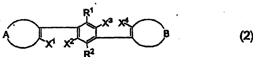
[Chem 4]
