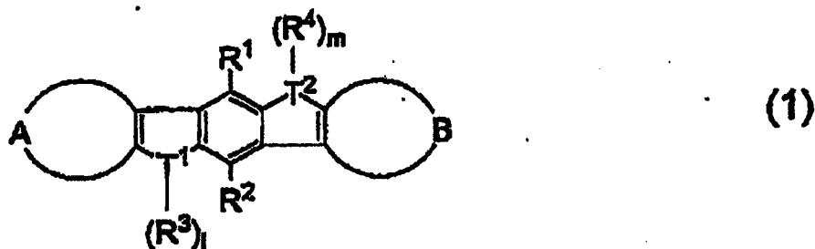
[Chem 8]
