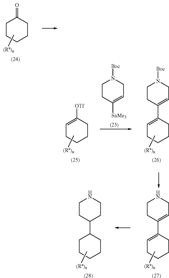
Scheme 6
