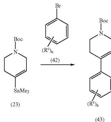
Scheme 10
