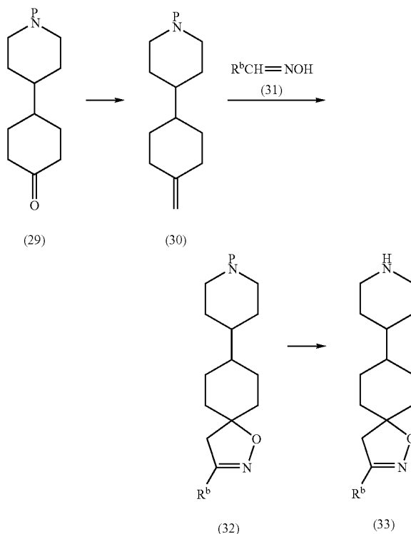
Scheme 7
