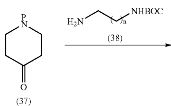
Scheme 9
