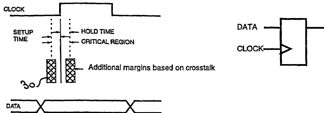
Figure 3., Static Timing analysis with crosstalk back-annotation
