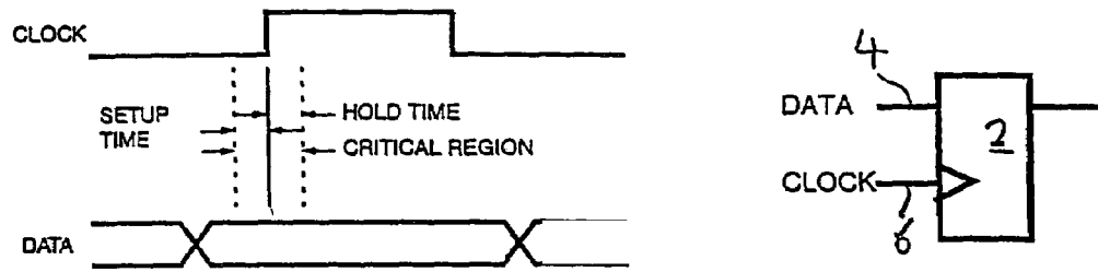
Figure 1. Traditional Static Timing analysis
