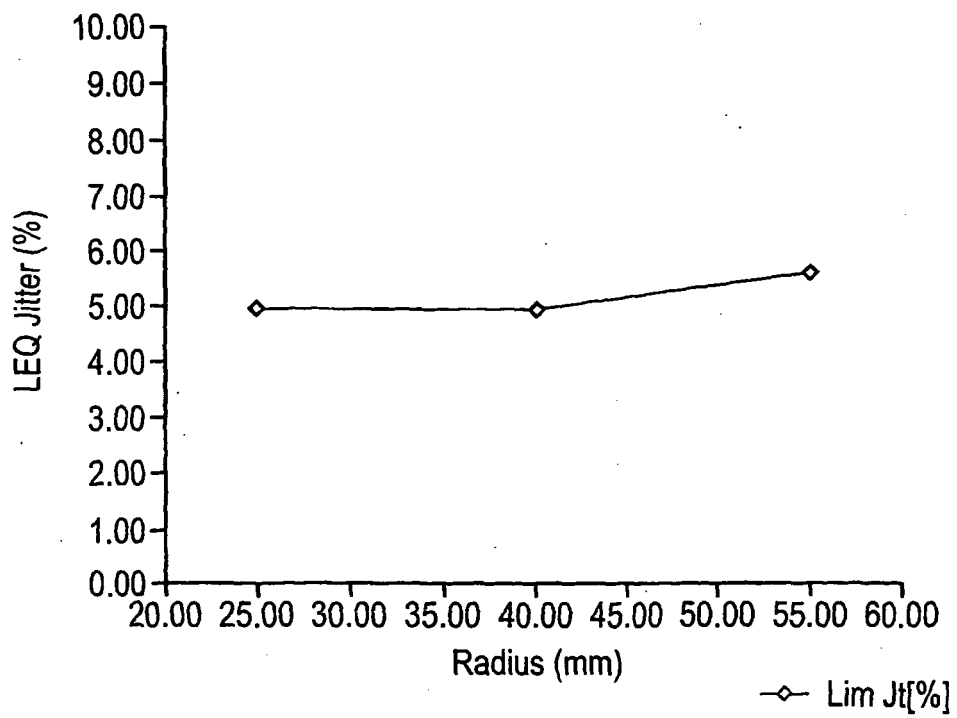
Electrical Signal Evaluation (Jitter)
