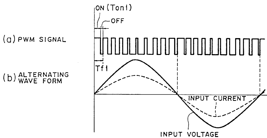
FIG. II PRIOR ART
