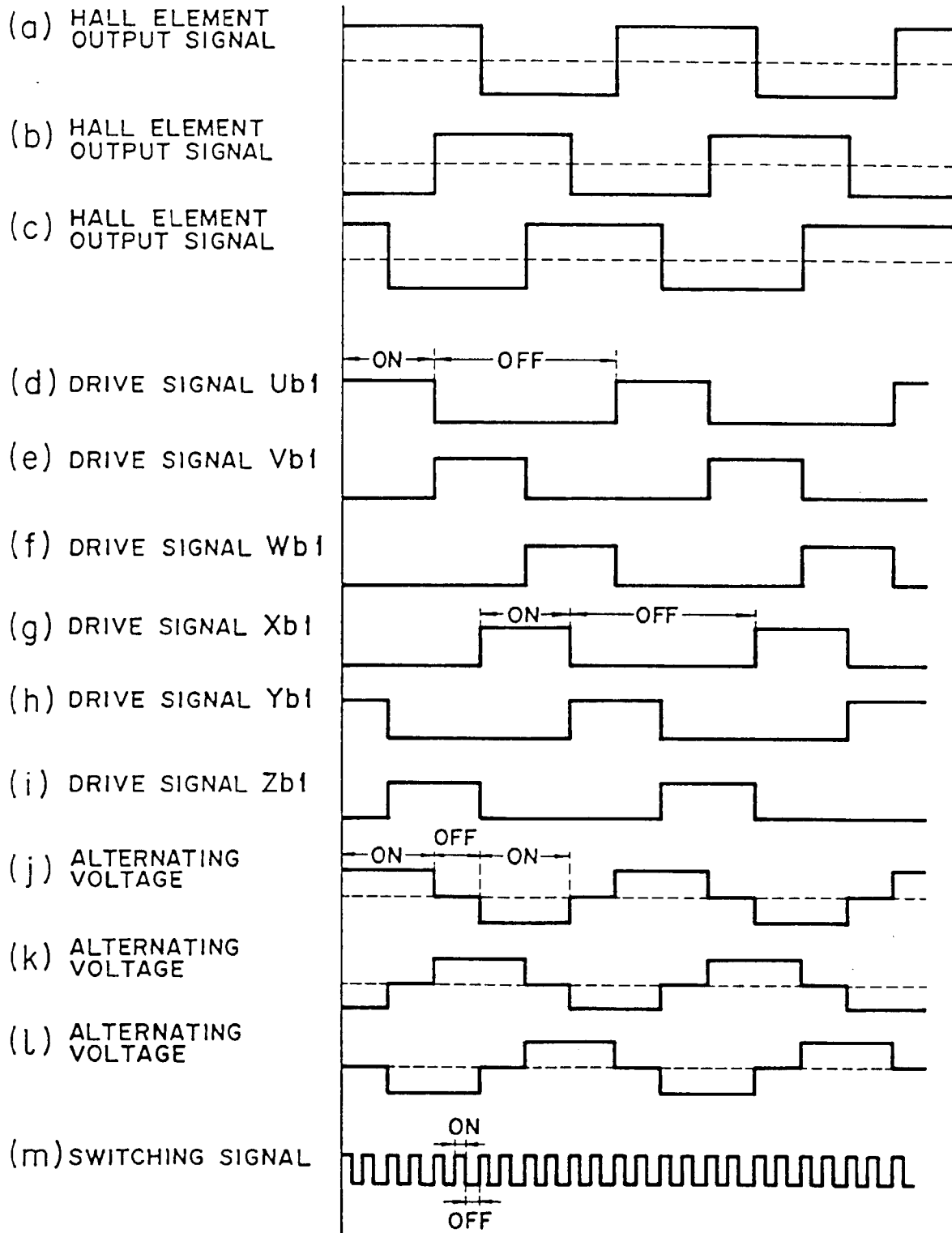
FIG. 13 PRIOR ART
