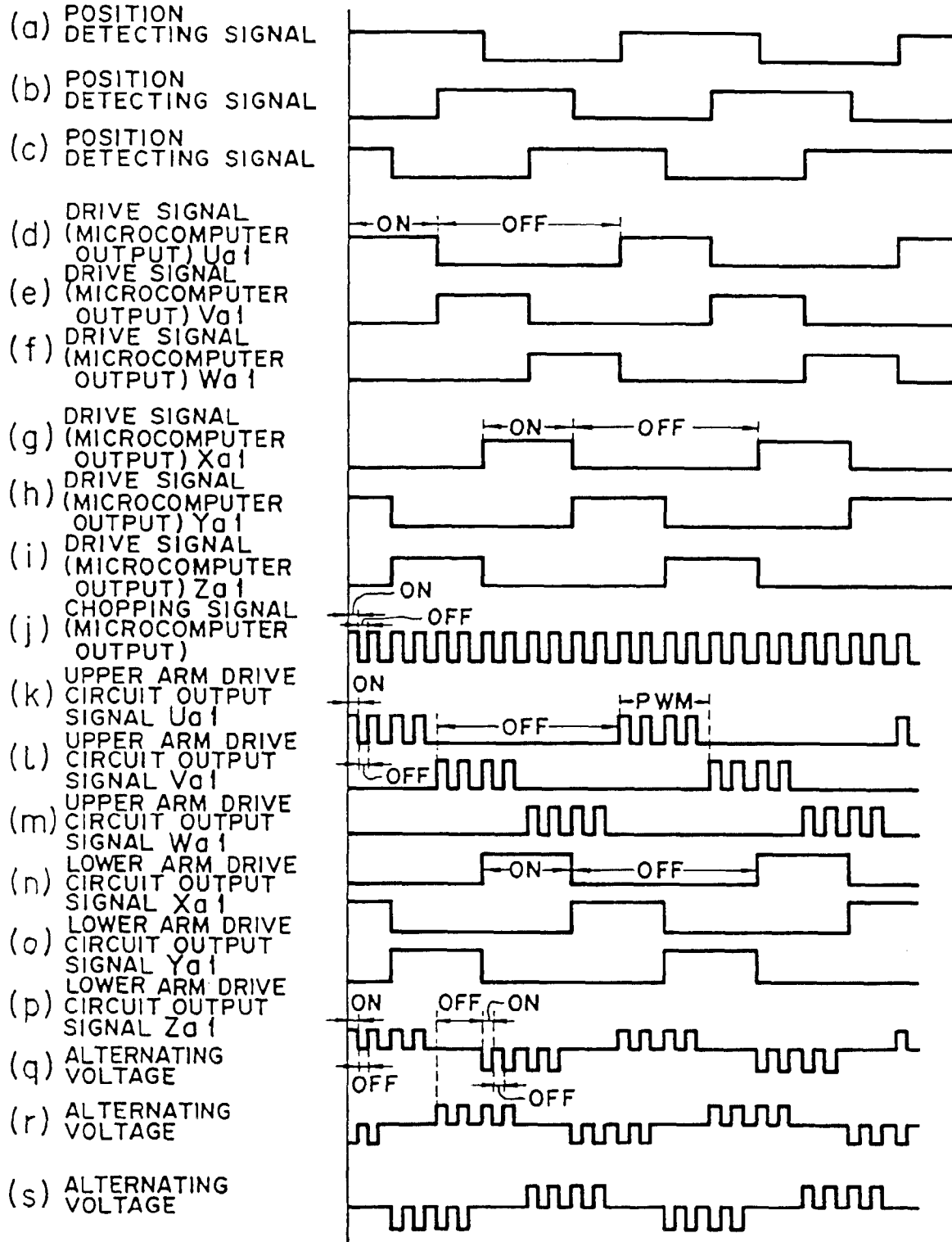
FIG. 12 PRIOR ART
