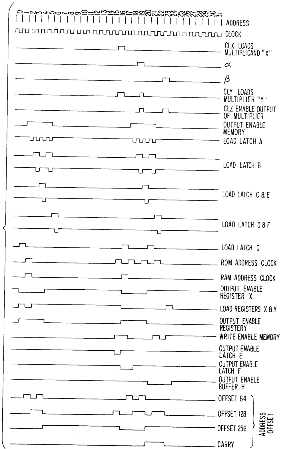
FIG 18 PROGRAM FOR CONTROL PROM
