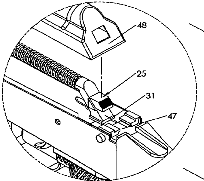
FIG 6 (Prior Art)
