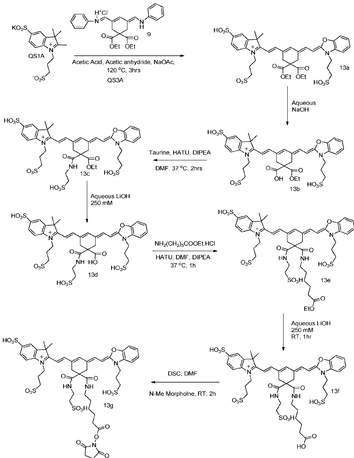
Scheme 3M. Synthesis of Asymmetric Indolinium - Bezoxazole Dye
