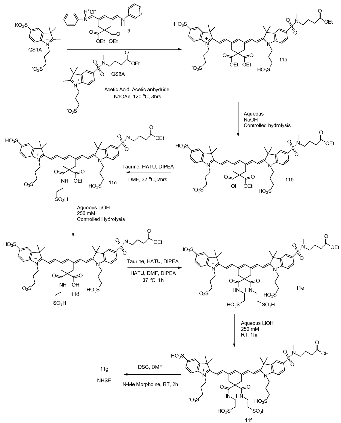
Scheme 3K. Synthesis of Asymmetric Indolinium Dye
