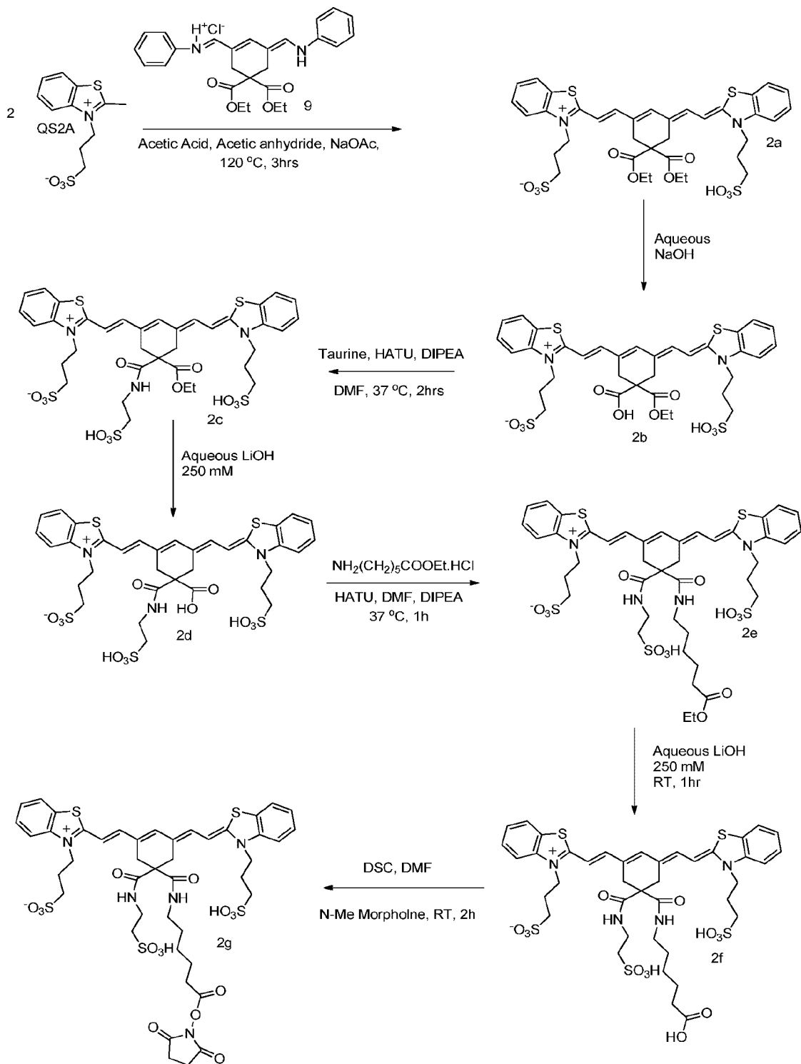
Scheme 3C. Synthesis of Symmetric Benzothiazolium Dye
