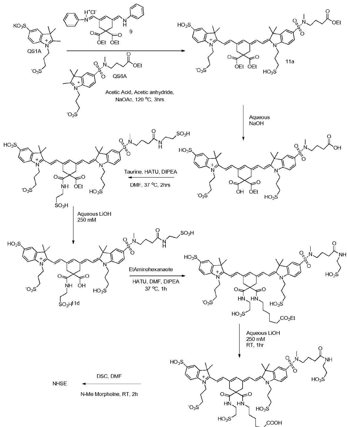
Scheme 3T. Synthesis of Asymmetric Indolinium Dye
