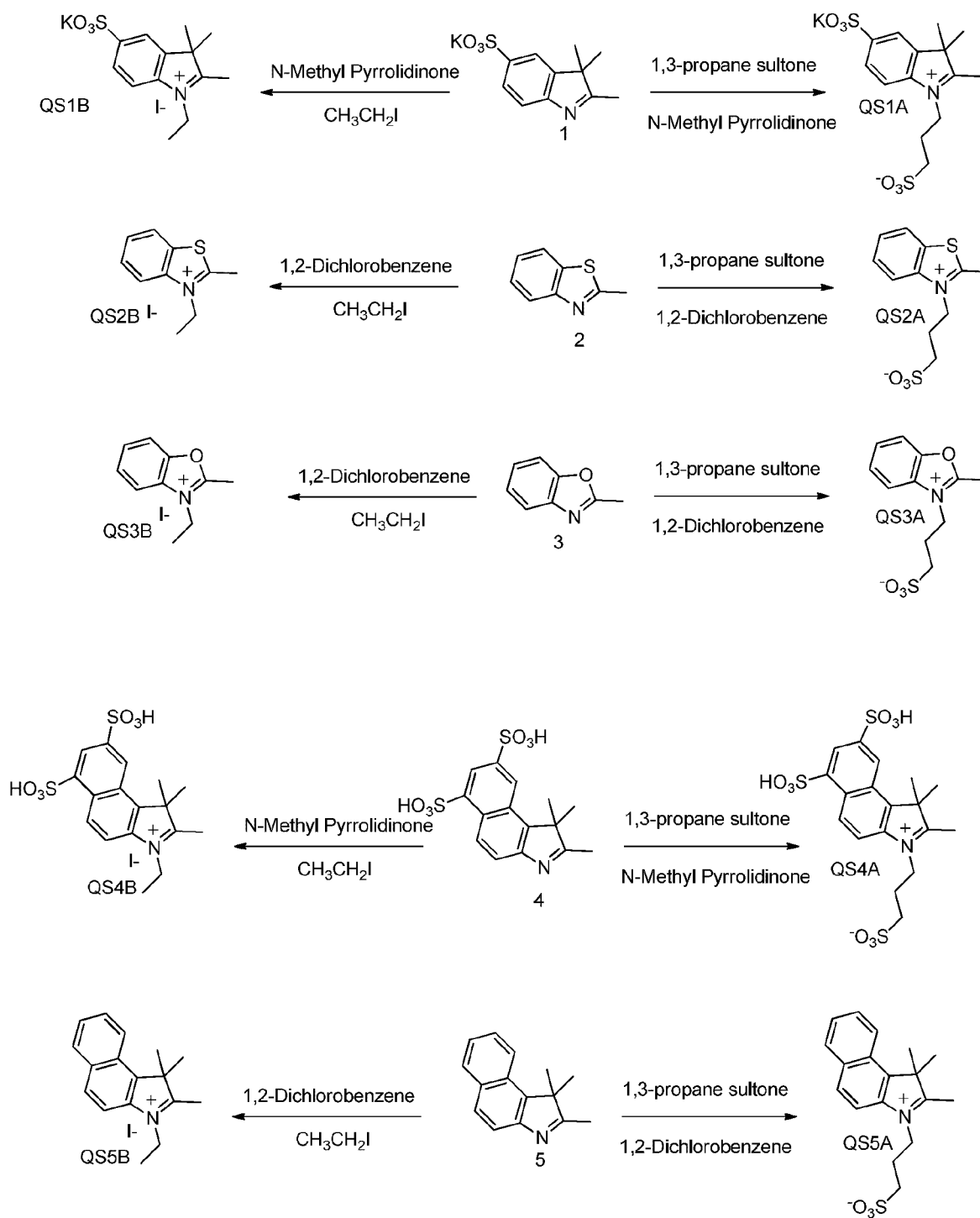
Scheme 1. Preparation of Quaternary Salts
