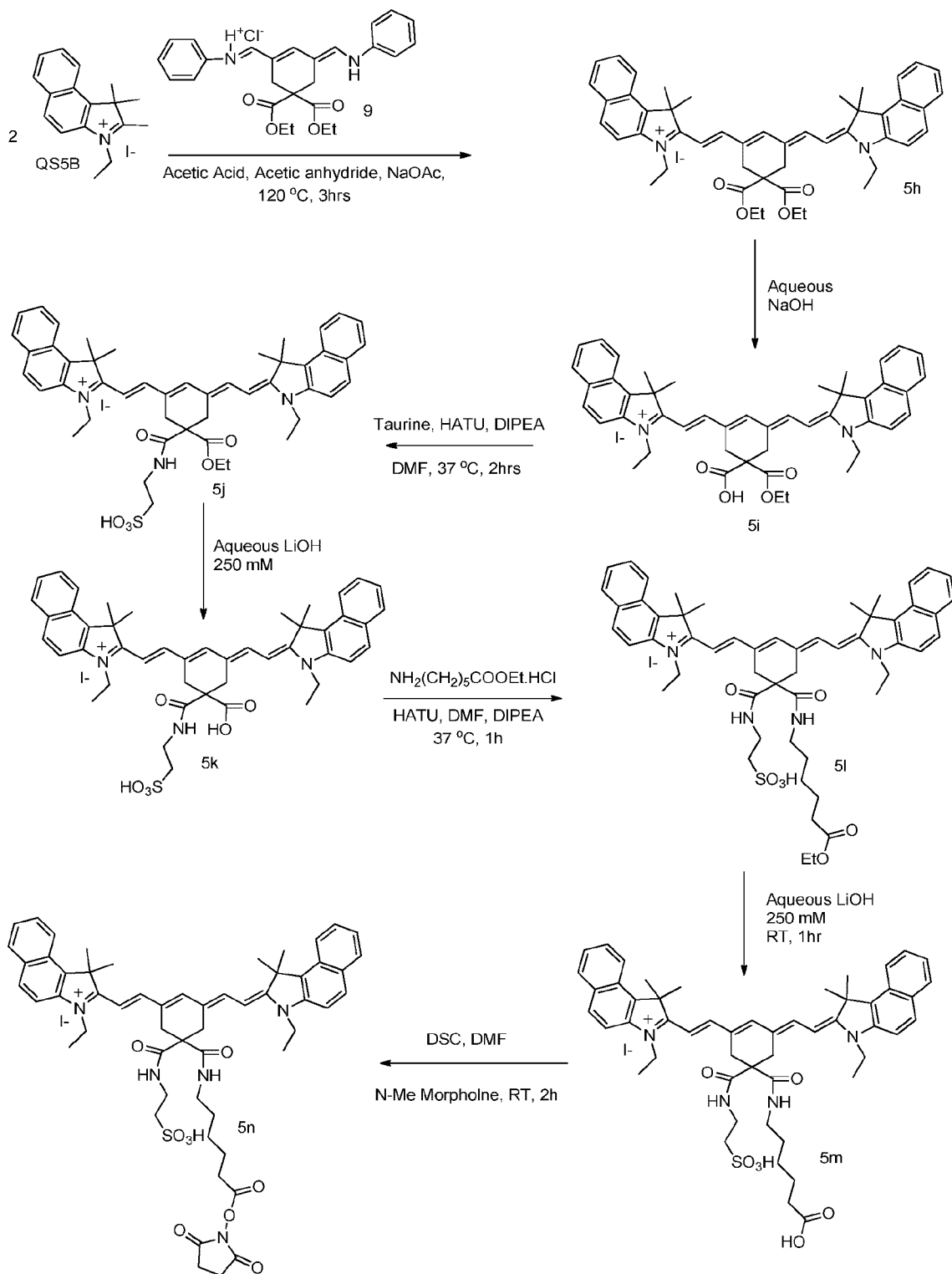
Scheme 3J. Synthesis of Symmetric Benzindole Dye
