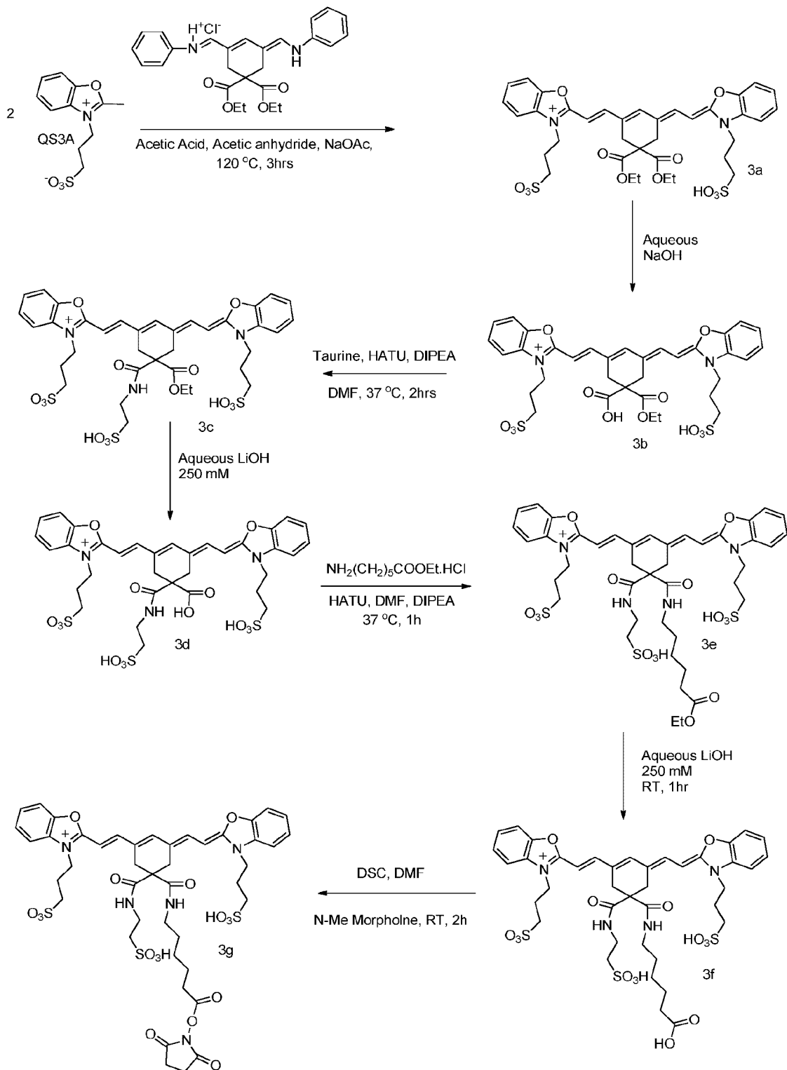
Scheme 3E. Synthesis of Symmetric Benzoxazole Dye
