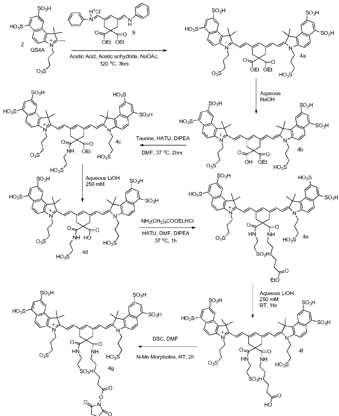
Scheme 3G. Synthesis of Symmetric Benzindole Dye
