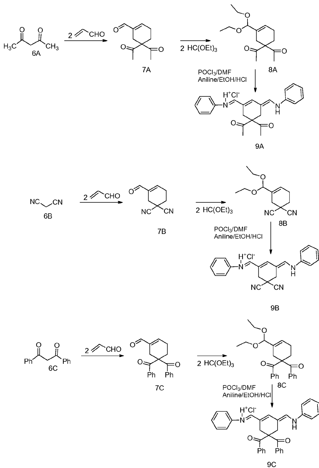
Scheme 2A. Preparation of Bridge
