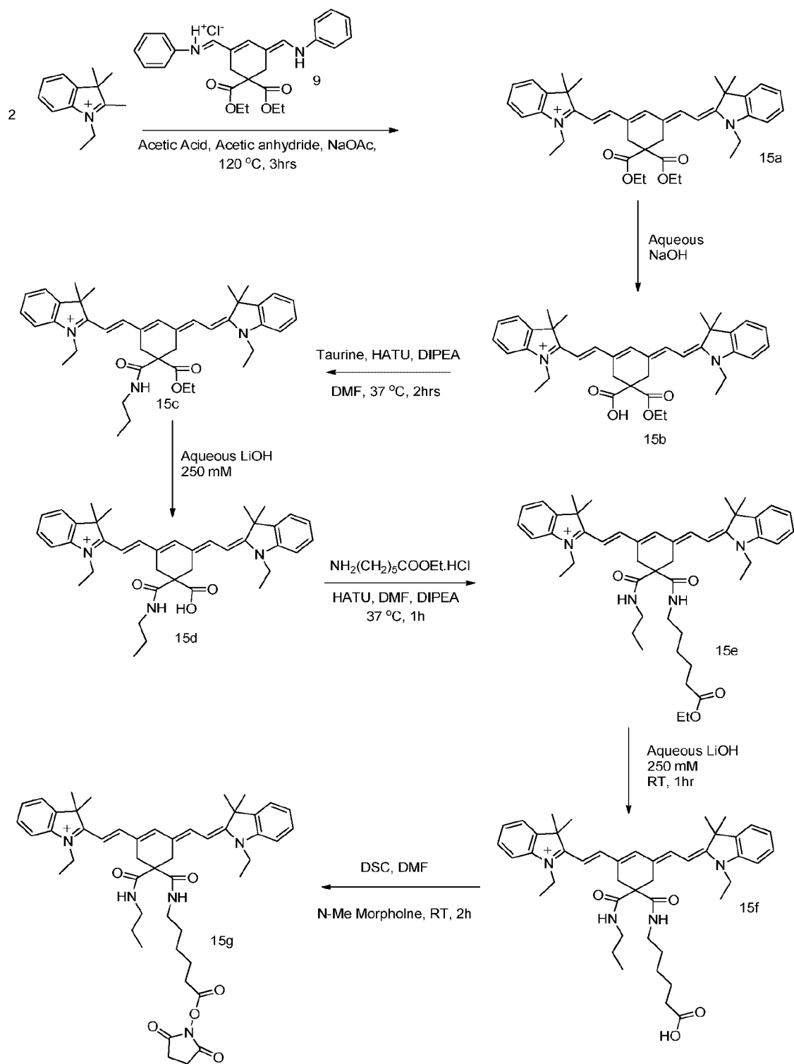
Scheme 3P. Synthesis of Symmetric Indolinium Hydrophobic Dye
