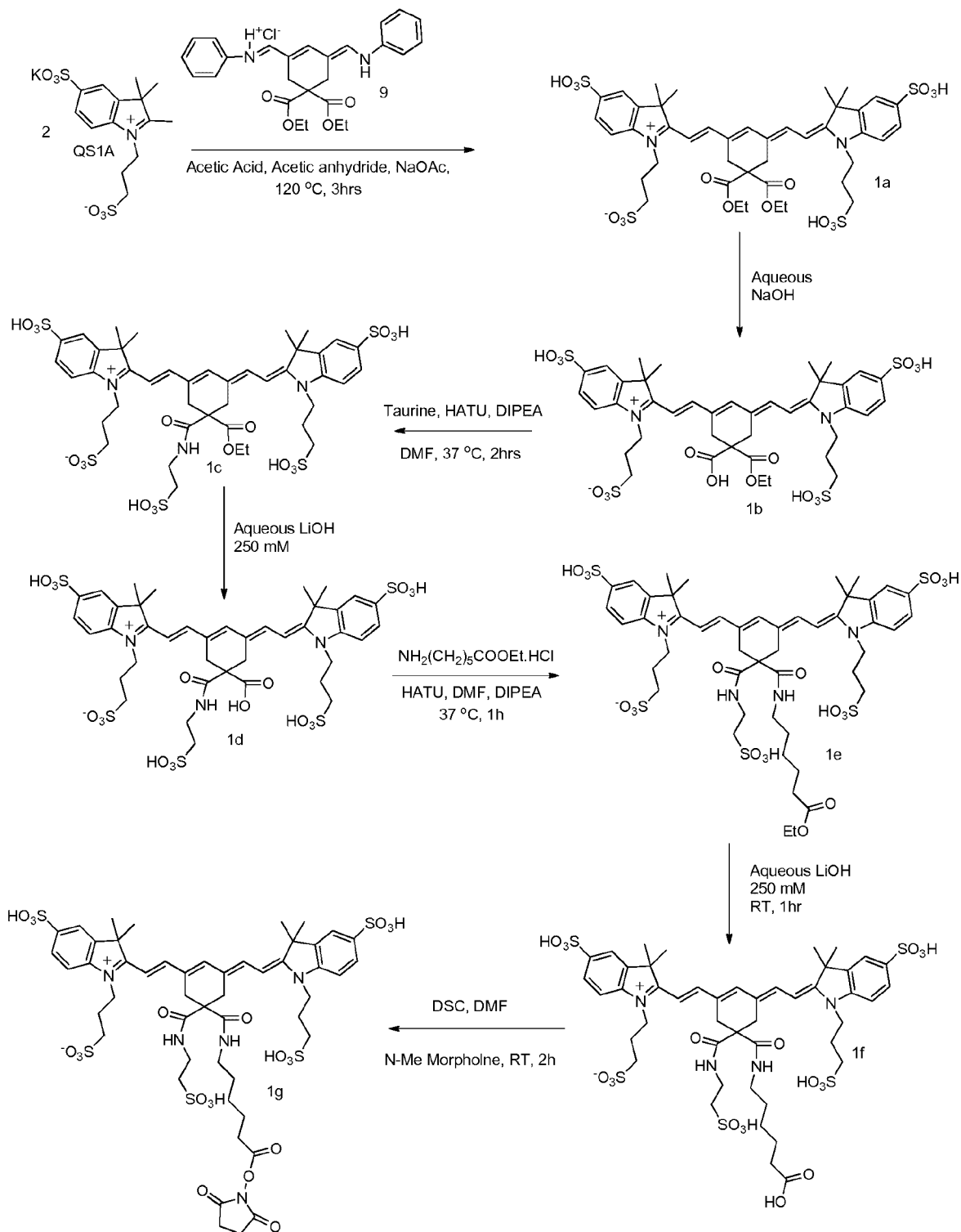
Scheme 3A. Synthesis of Symmetric Indolinium Hydrophilic Dye
