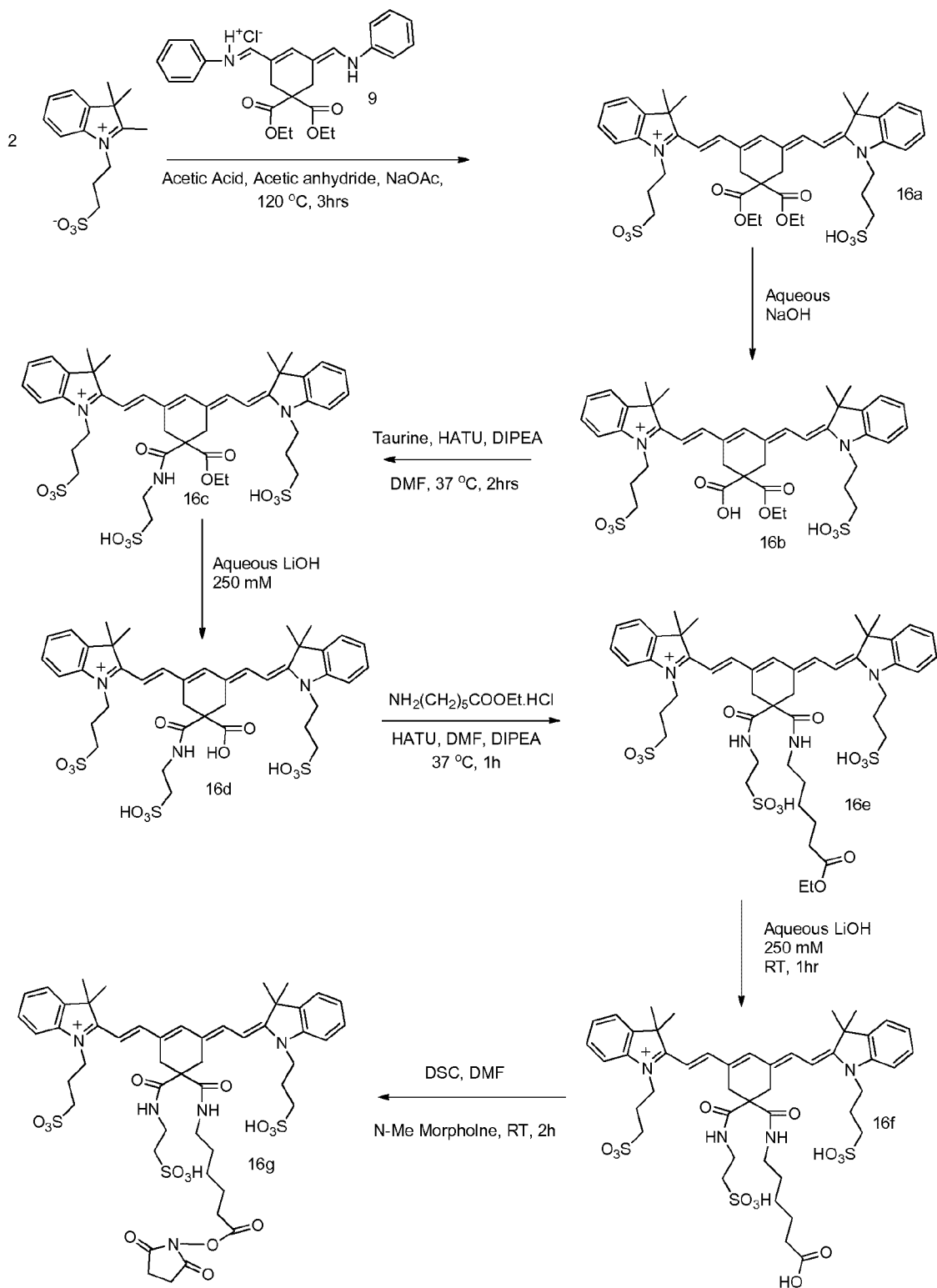
Scheme 3Q. Synthesis of Symmetric Indolinium Dye
