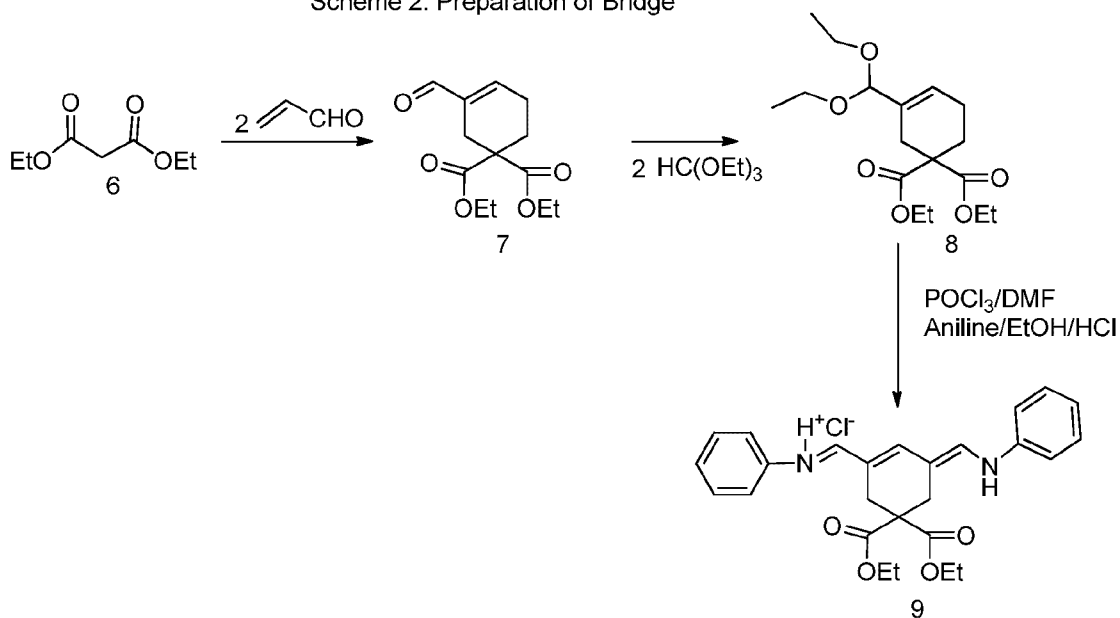
Scheme 2. Preparation of Bridge
