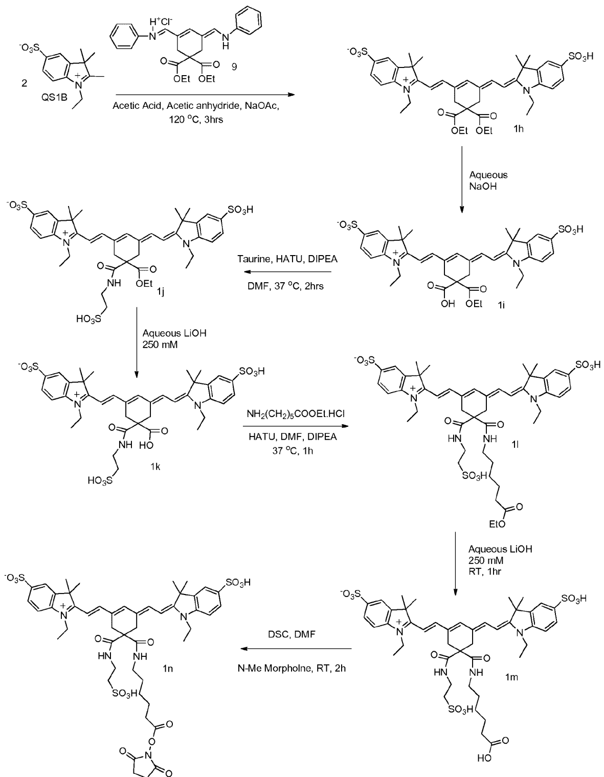
Scheme 3B. Synthesis of Symmetric Indolinium Dye
