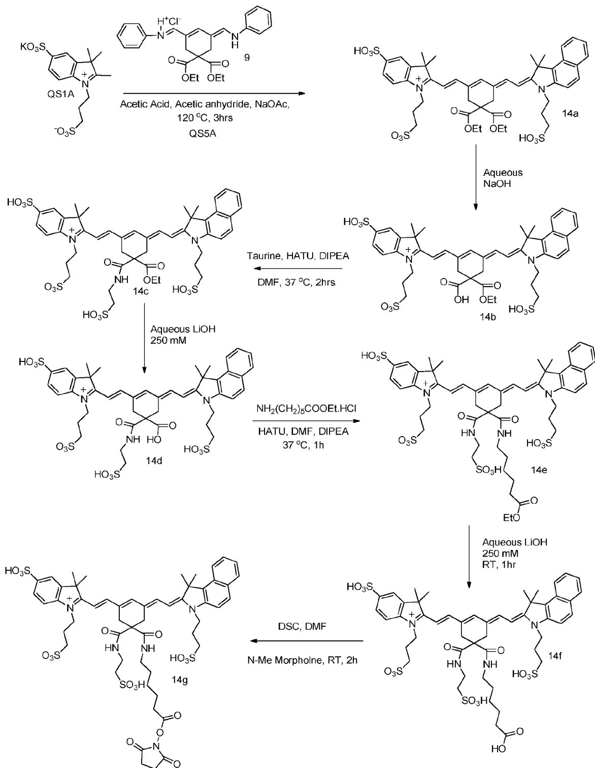
Scheme 3N. Synthesis of Asymmetric Indolinium - Benzindolium Dye
