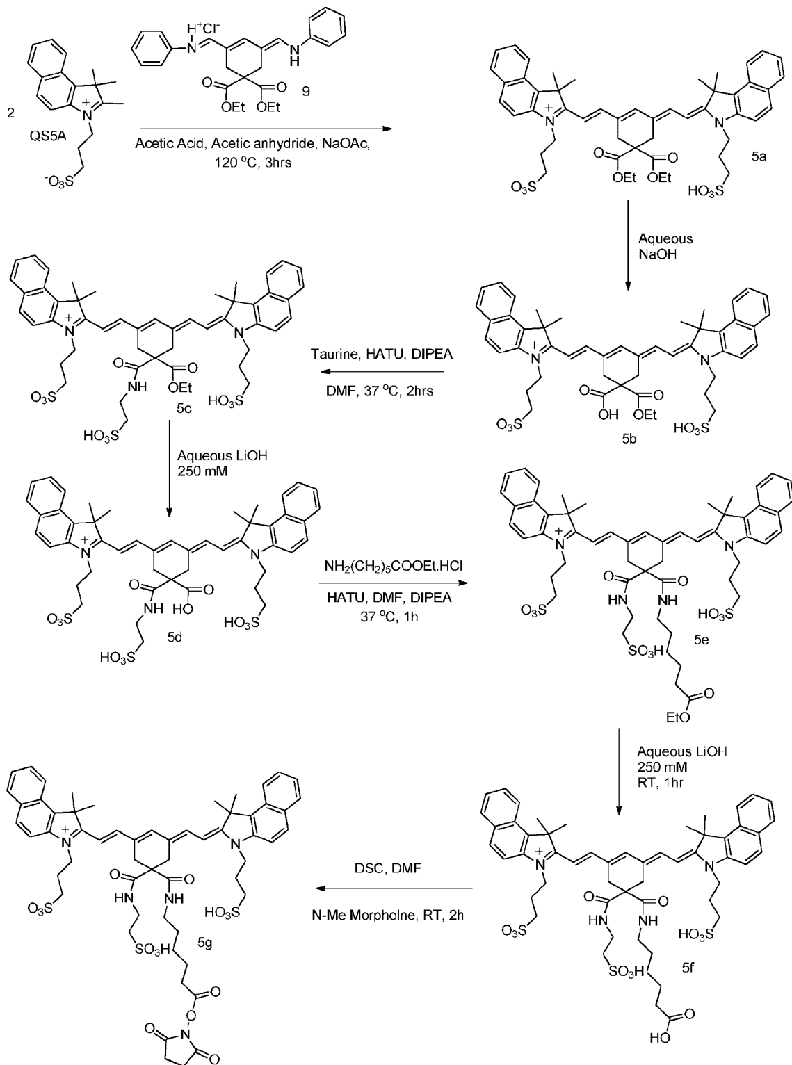
Scheme 3I. Synthesis of Symmetric Benzindole Dye
