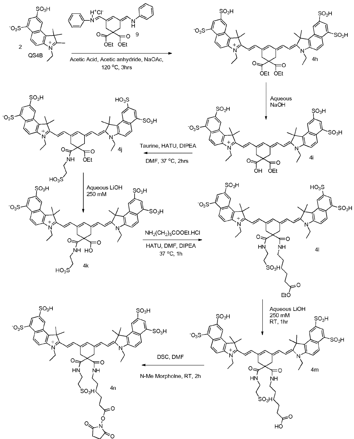
Scheme 3H. Synthesis of Symmetric Benzindole Dye
