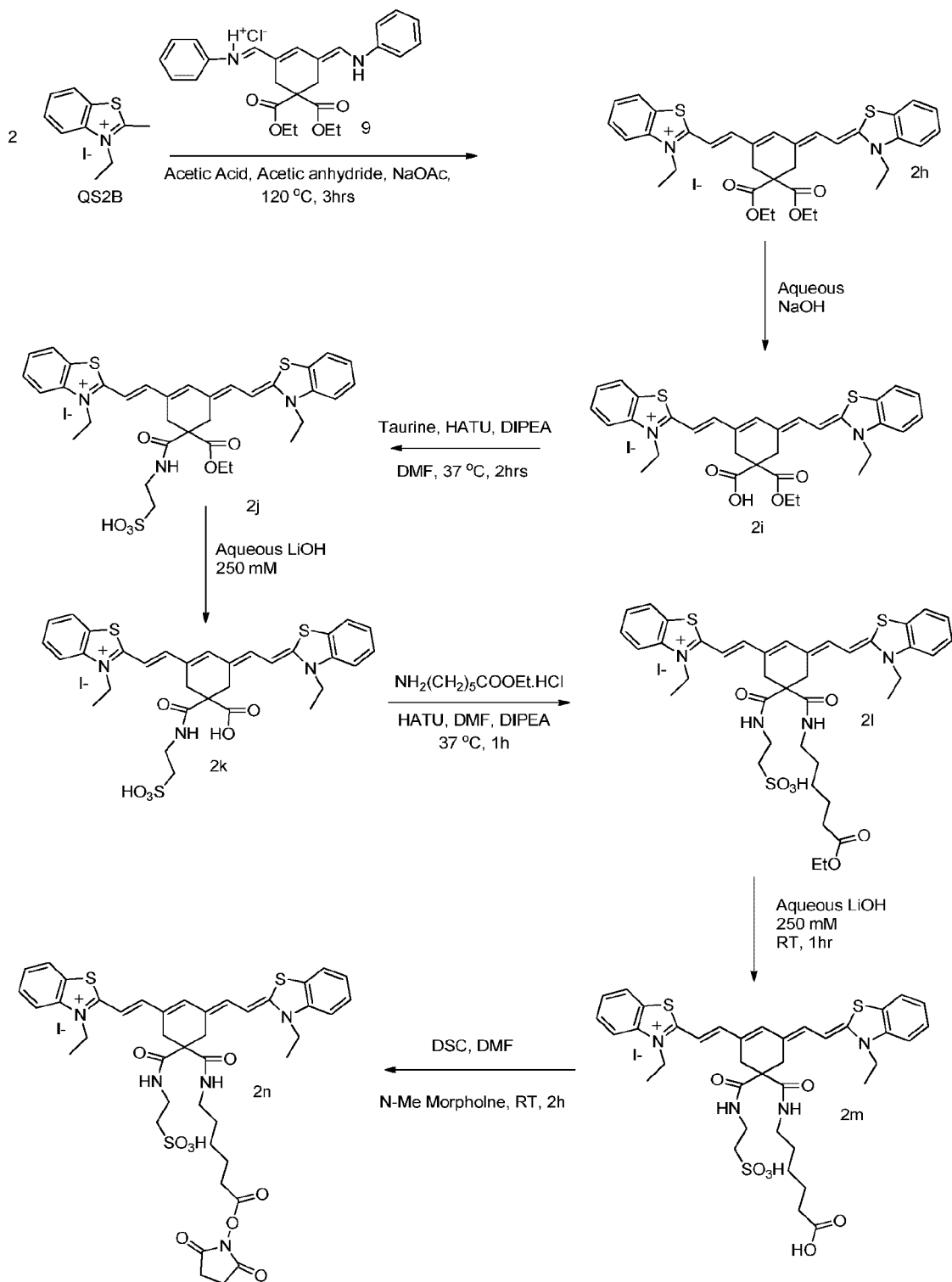
Scheme 3D. Synthesis of Symmetric Benzothiazolium Dye
