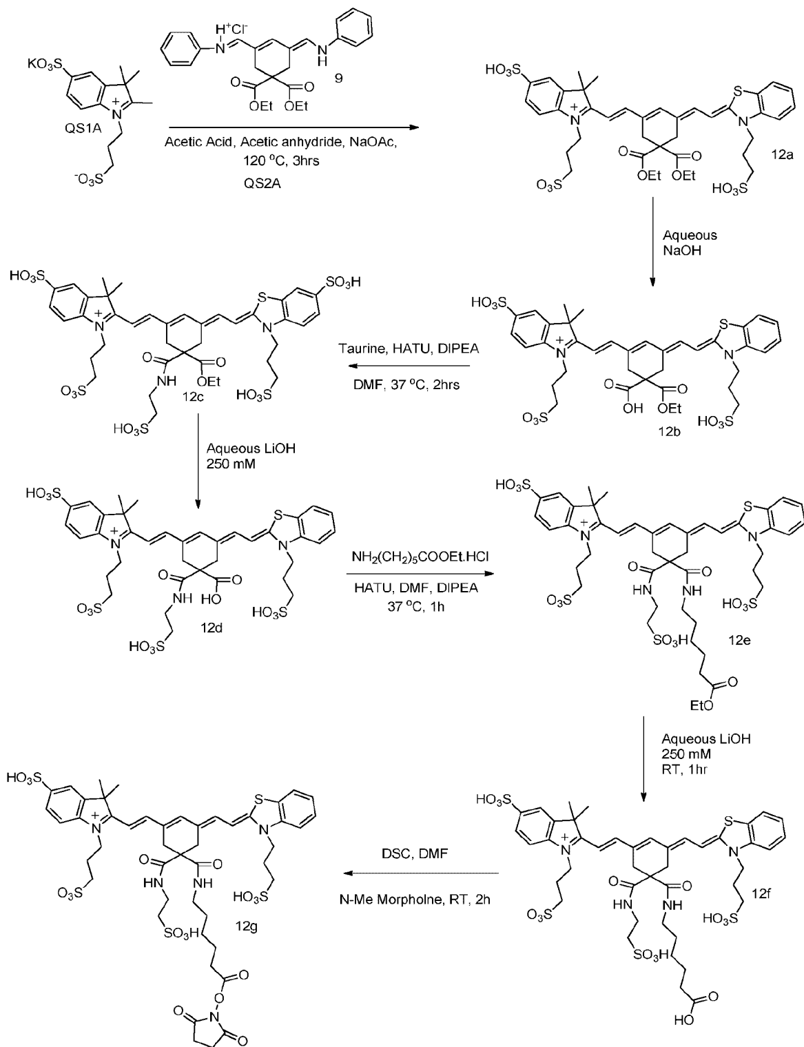
Scheme 3L. Synthesis of Asymmetric Indolinium-Benzothiazole Dye
