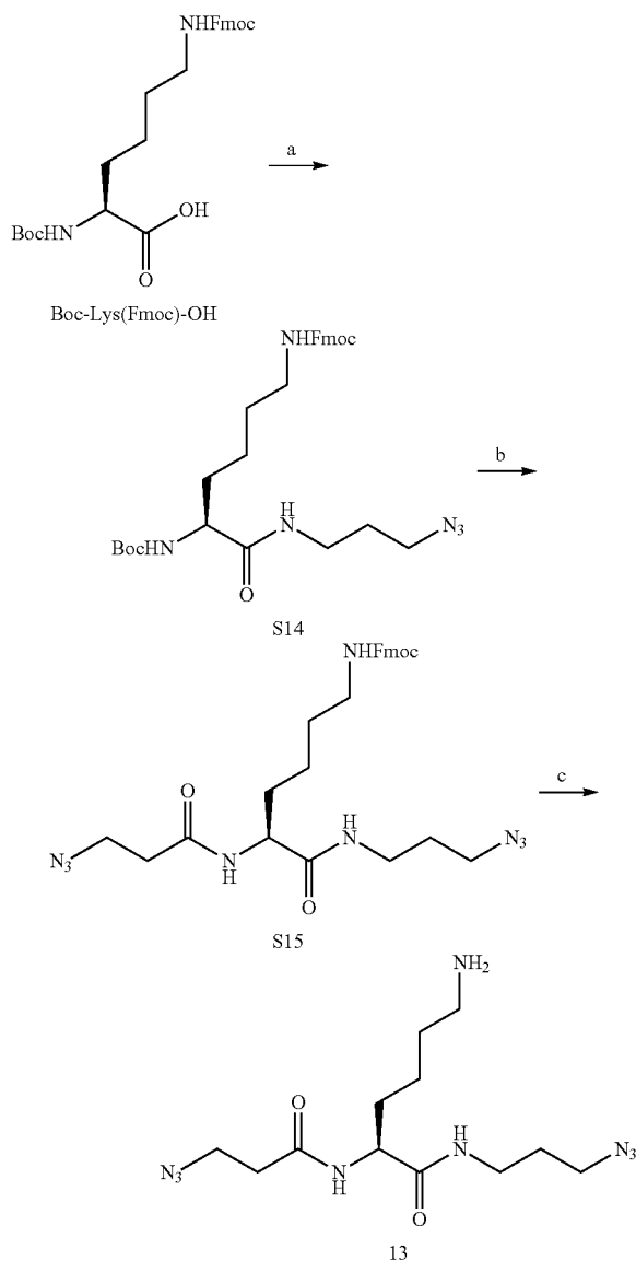
Scheme 9. Synthesis of branched linker 13.
