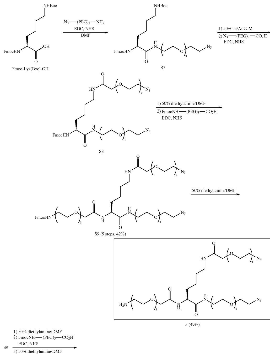
Scheme 7. Synthesis of branched linker compounds 5-7.
