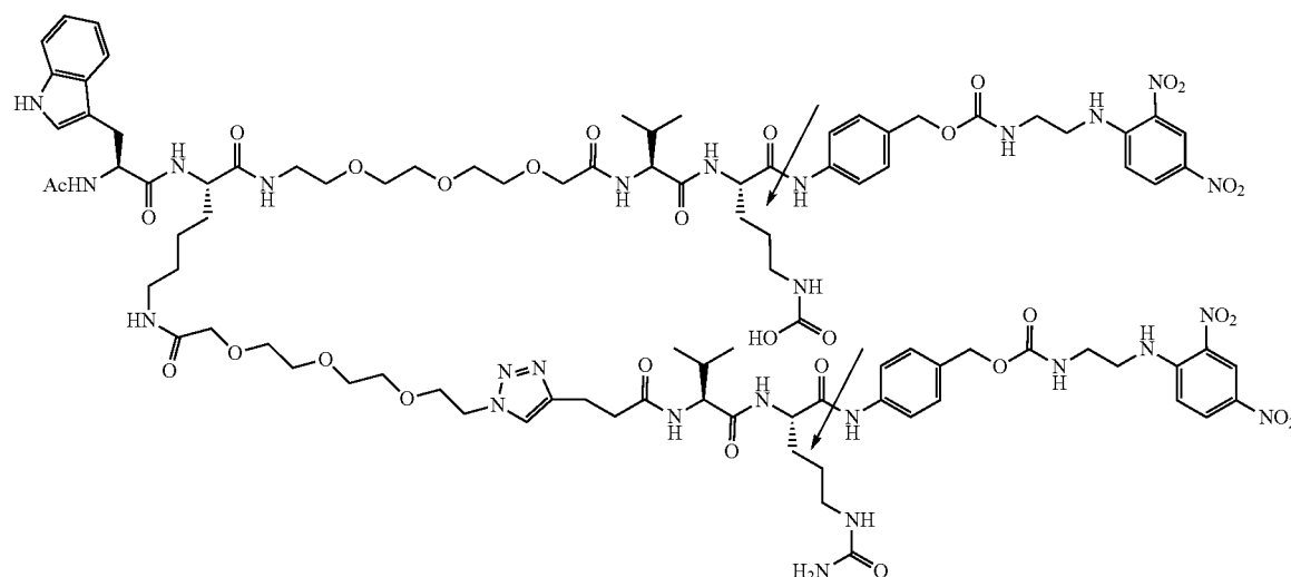
Structures of fluorescent probes 1-4 containing tryptophan (fluorophore) and EdDnp groups (quencher) for the FRET assay (See the Examples below for synthesis detail). The Val-Cit sequence undergoes cathepsin B-mediated cleavage (depicted with an arrow) to release the EdDnp from the probes, enabling fluorescence detection derived from the tryptophan (excitation: 280 nm, emission: 360).
