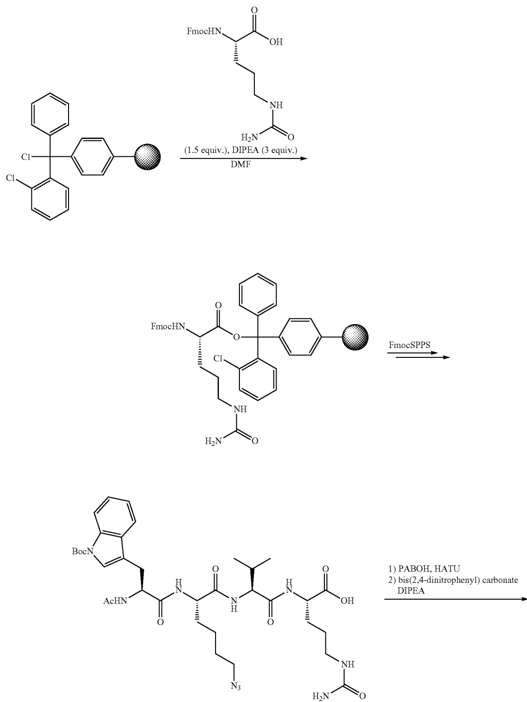
Scheme 3. Synthesis of linear probe 1.
