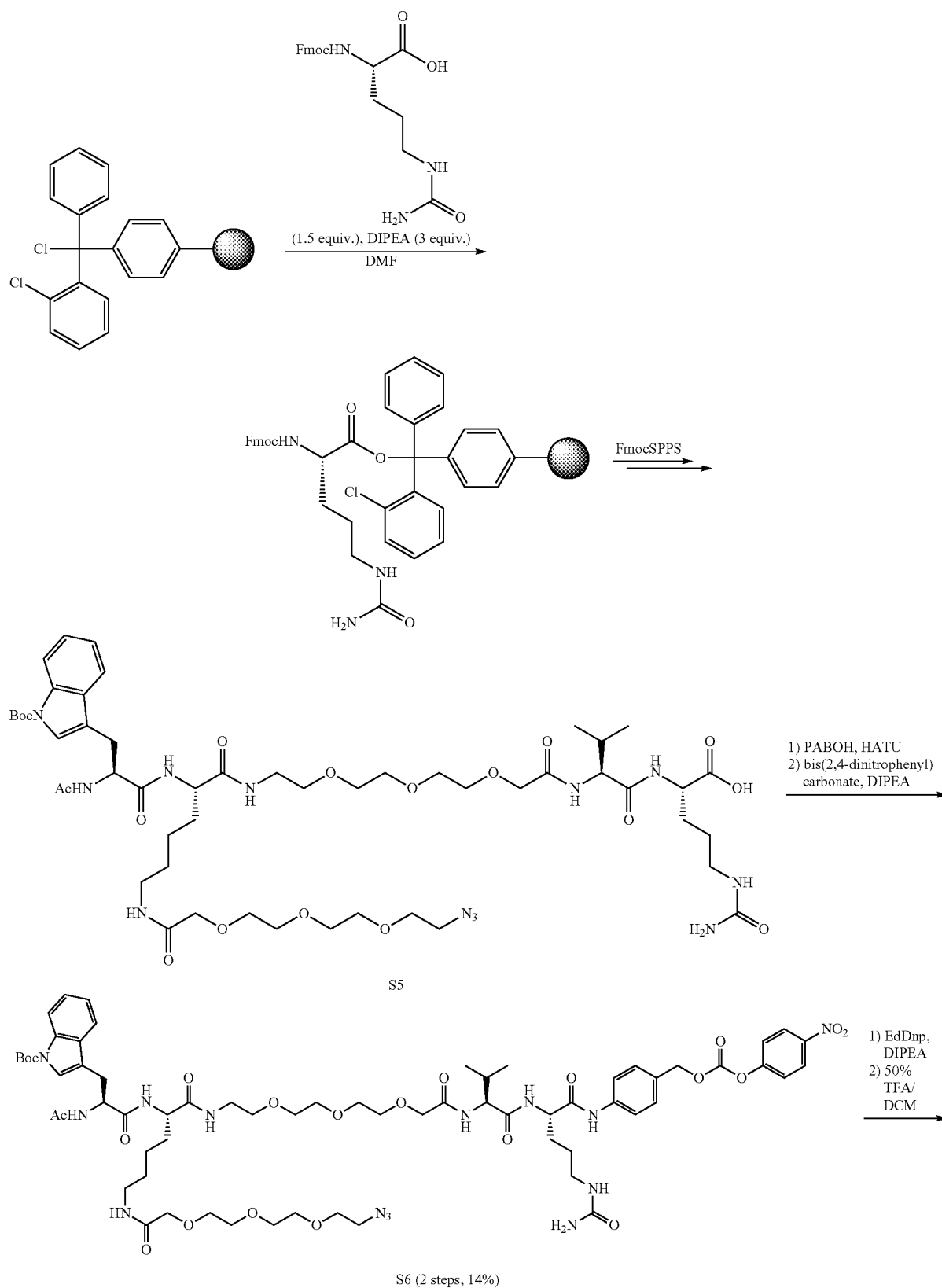
Scheme 5. Synthesis of linear probe containing PEG spacer 2.
