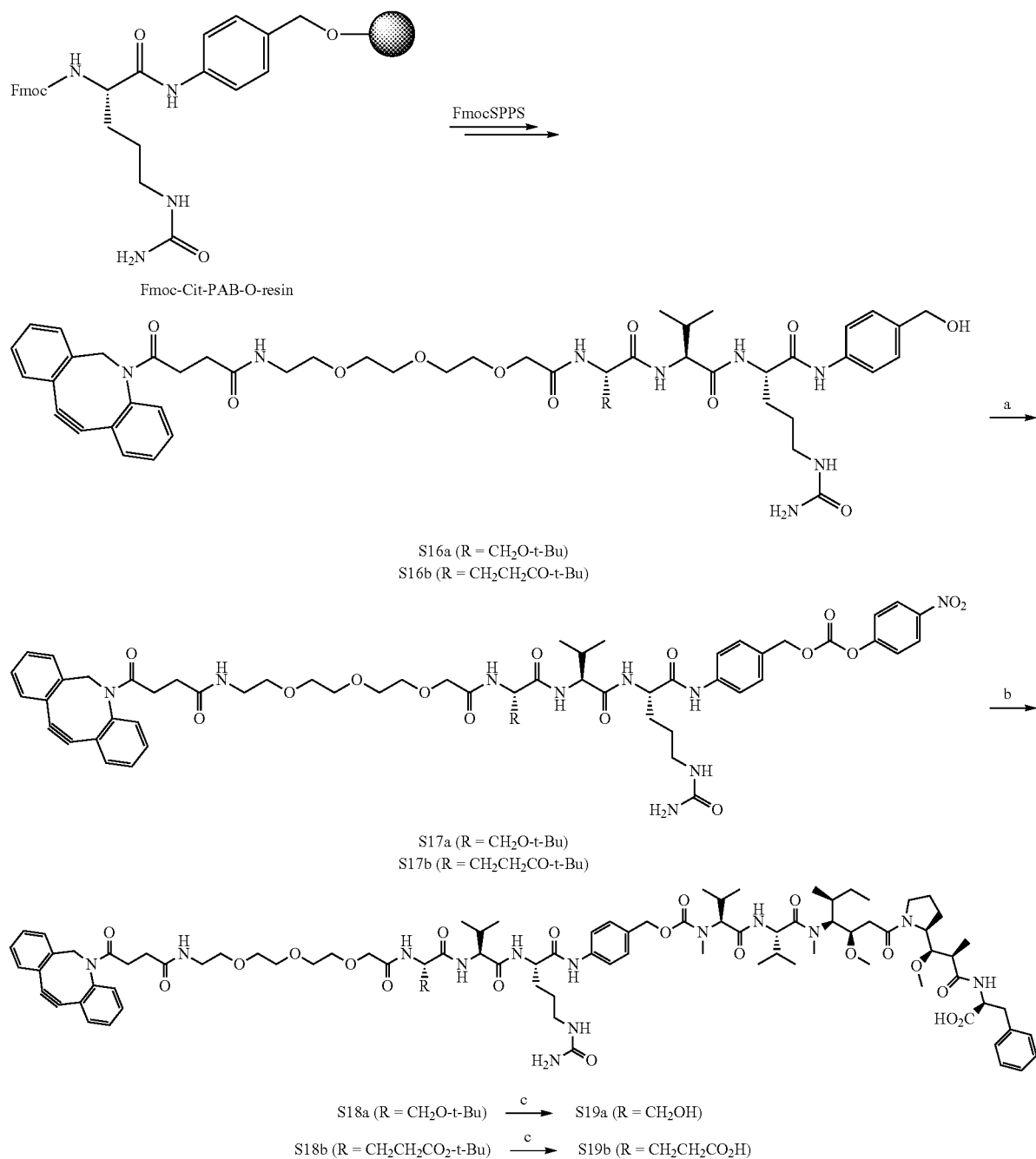
Scheme 10. Synthesis of DBCO-MMAF fragments S19a and S19b.
