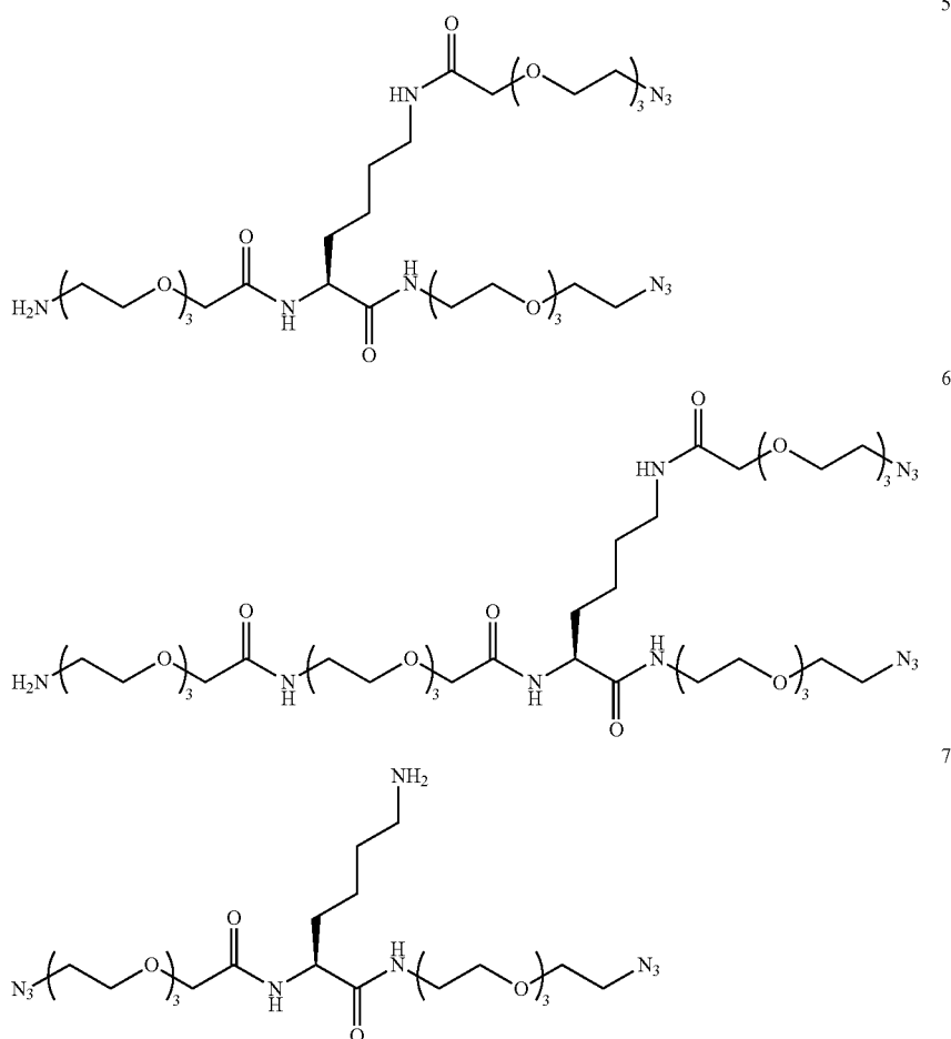
Scheme 2. Structures of branched linkers 5-7.
