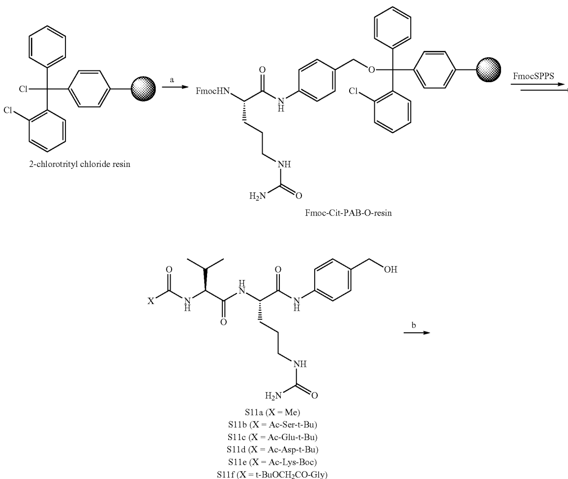
Scheme 8. Synthesis of pyrene probes 12a-f.
