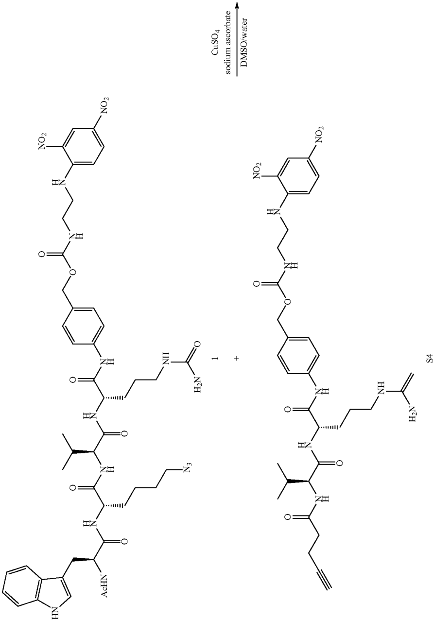
Scheme 6. Synthesis of branched probes 3 and 4.
