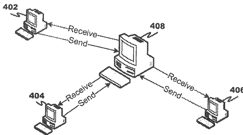
Client-Server Architecture
