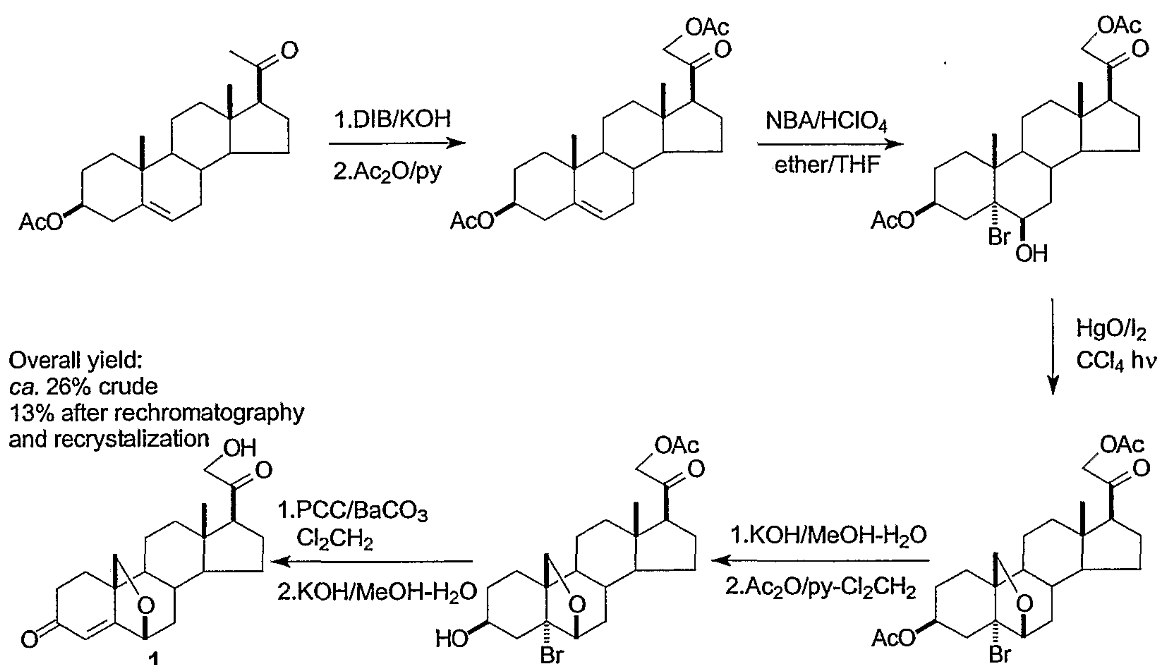
Scheme 3: Synthesis of 21-hydroxy-6,19-oxidoprogesterone by Veleiro et al.
