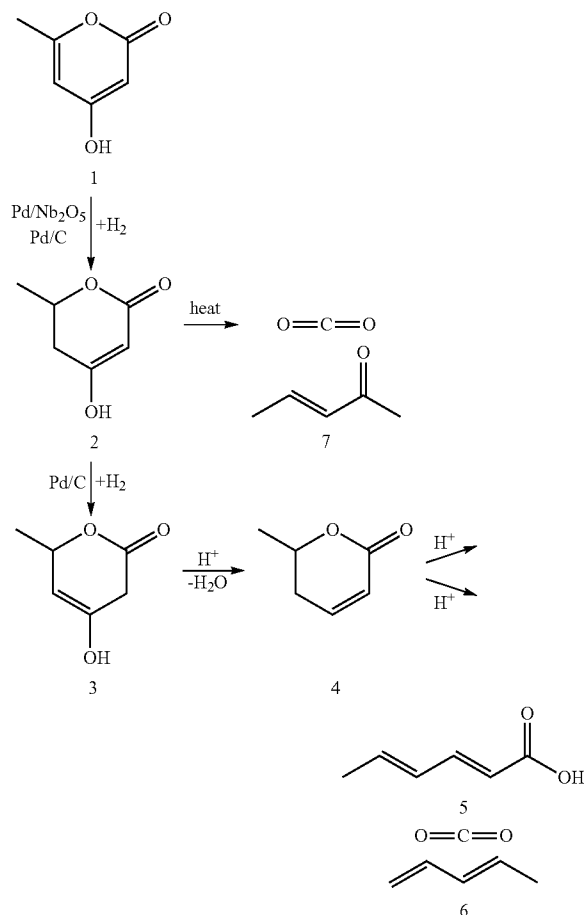
Reaction Scheme 1
