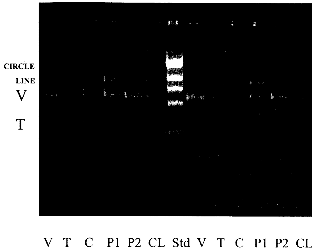
Fig. 4. Ribocloning the Taq gene
