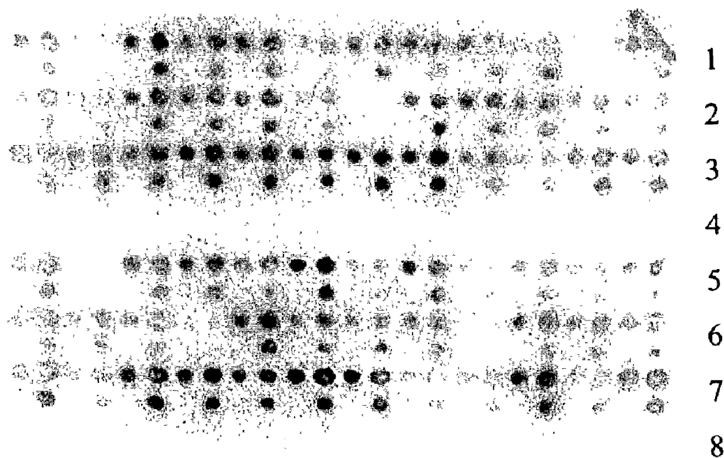
Fig. 6. Colony assay for thermostable DNA polymerase activity.
