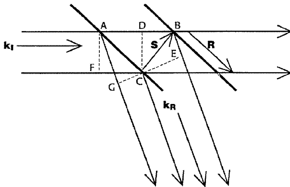
Fig. 11 - Array reflector spacing and orientation
