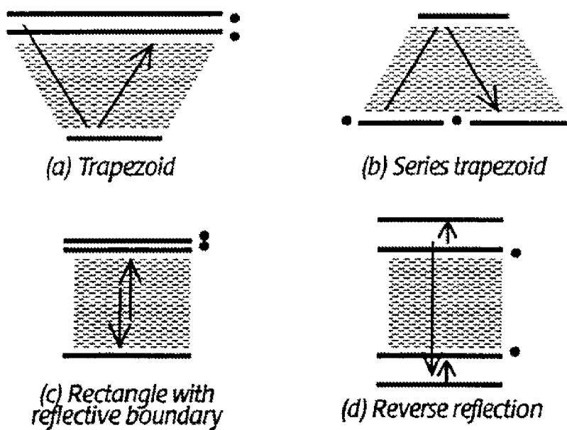
Fig. 18 - Example touch region boundaries
