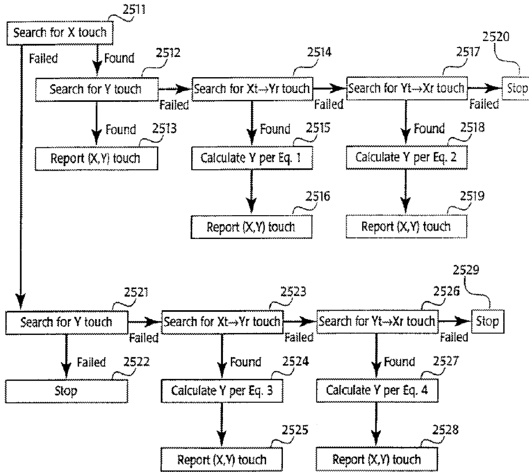
Fig. 25(b) Anti-Shadowing Algorithm Flow Chart
