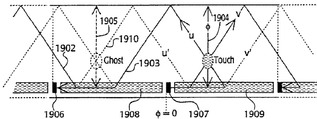
(b) "Planar" sensor with periodic extensions
