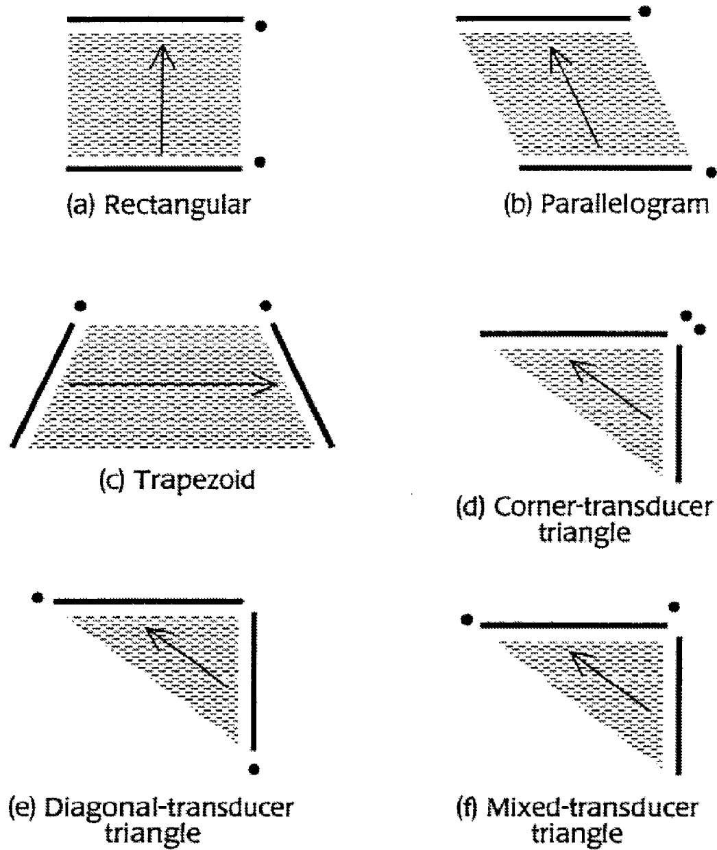
Fig. 12 - Example touch region geometries
