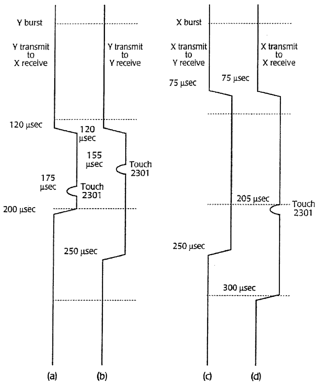
Fig. 23 - Example signals of sensor in Fig. 13
