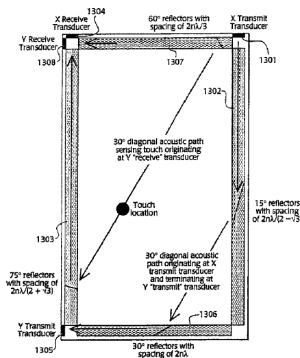
V Subsystem of X,Y,U,V Sensor
