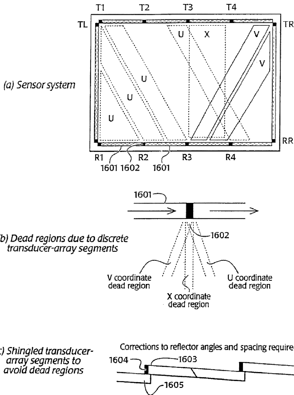
Fig. 16 - Large rectangular sensor
