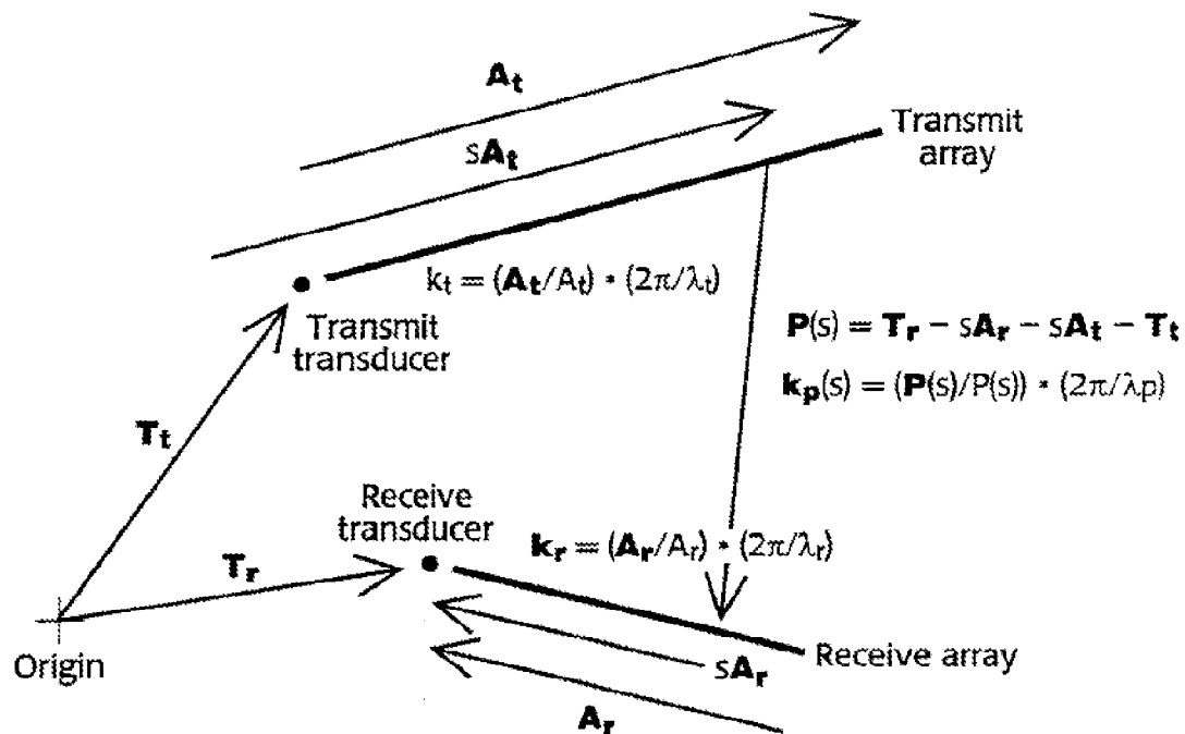
Fig. 10 - Planar coordinate subsystem
