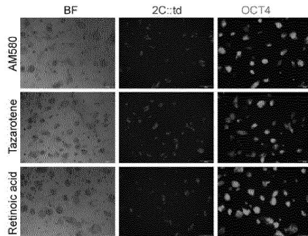
Substitution TTNPB with RA signaling pathway agonist
