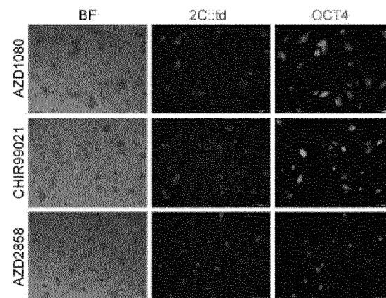
Substitution 1-Azakenpaullone with GSK3 signaling pathway inhibitor
