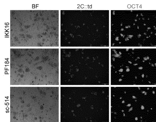
Substitution WS6 with IKK signaling pathway inhibitor
