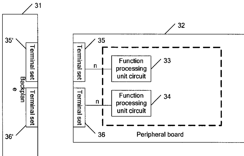
Fig. 3 (Related Art)
