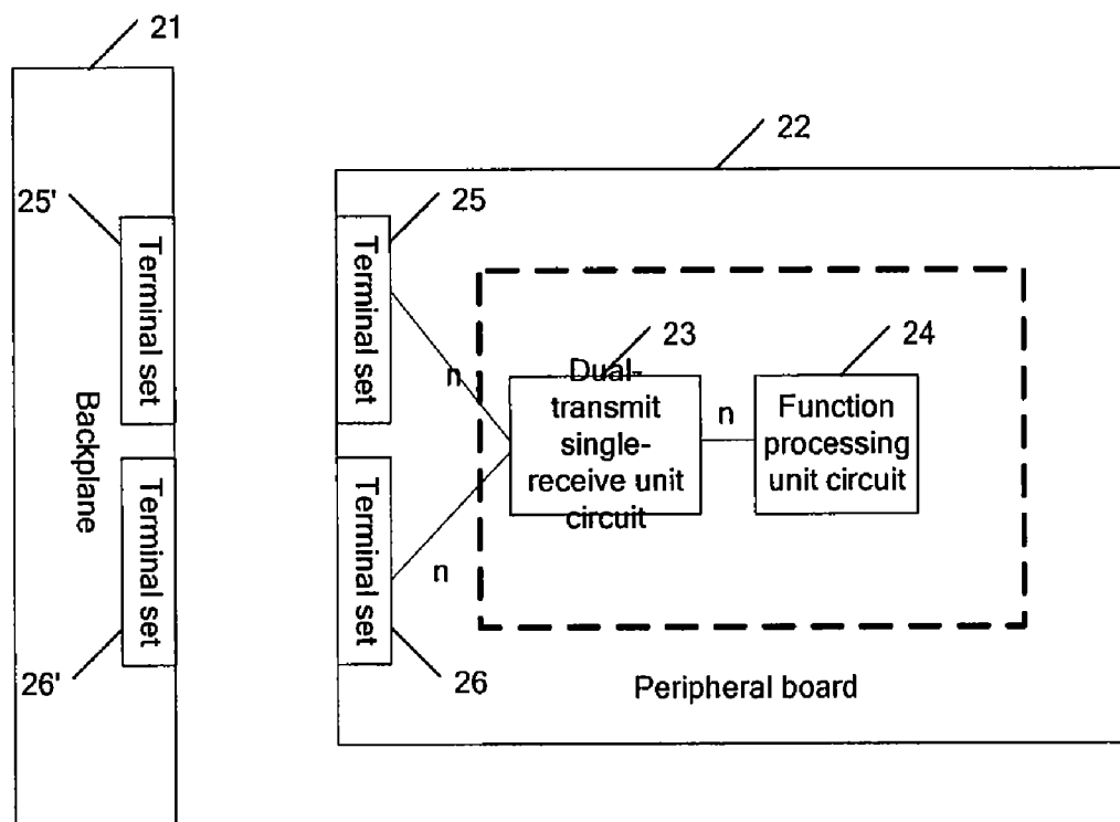
Fig.2 (Related Art)
