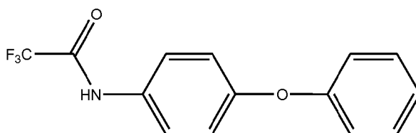
2,2,2-trifluoro-N-(4-phenoxyphenyl)acetamide
