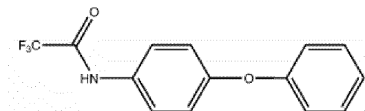
2,2,2-Trifluor-N-(4-phenoxyphenyl)acetamid
