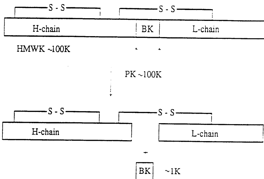
Figure 1. Cleavage of HMWK by PK: Overall scheme
