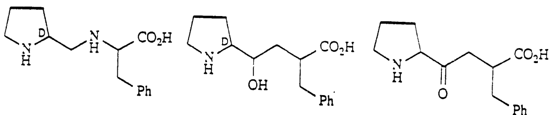
(i) 'Reduced' mimic (ii) 'Hydroxy' or hydroxyethylene mimic (iii) 'Keto' or ketomethylene mimic
