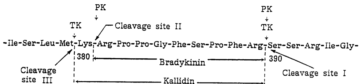
Figure 1. Cleavage of HMWK by PK: Overall scheme
