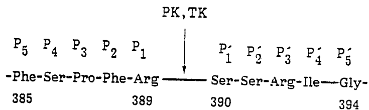
Figure 3. Sequences flanking cleavage site I in human HMWK
