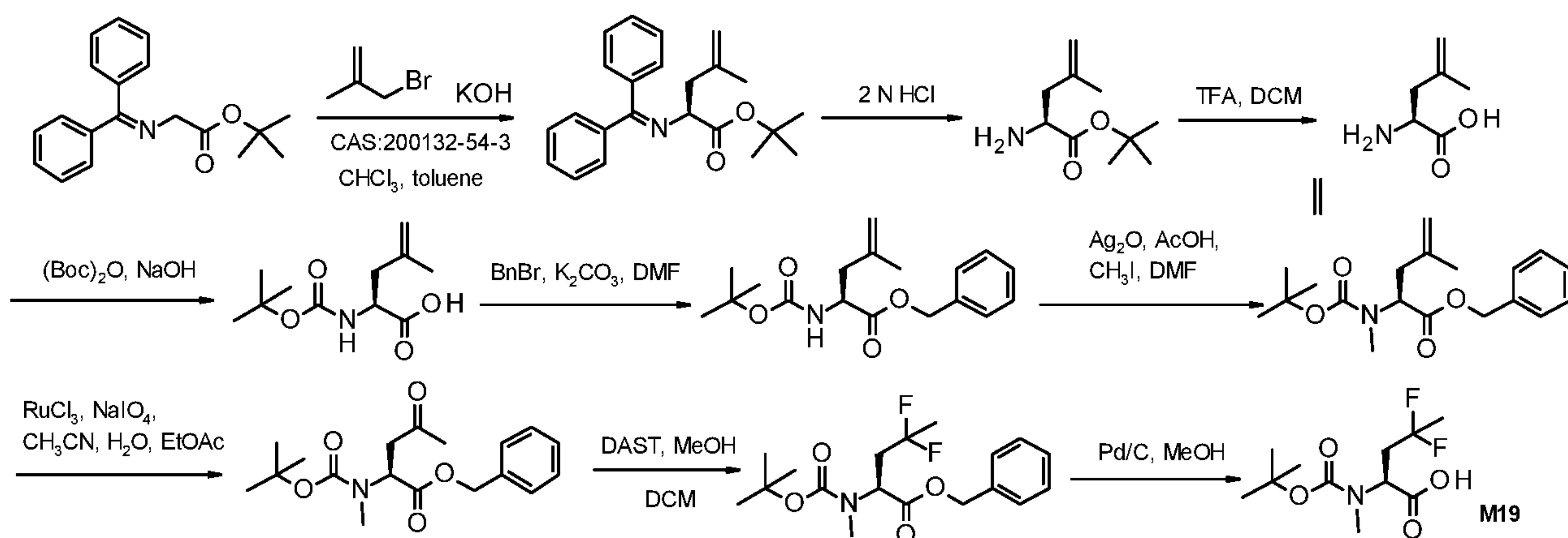
Scheme 12
