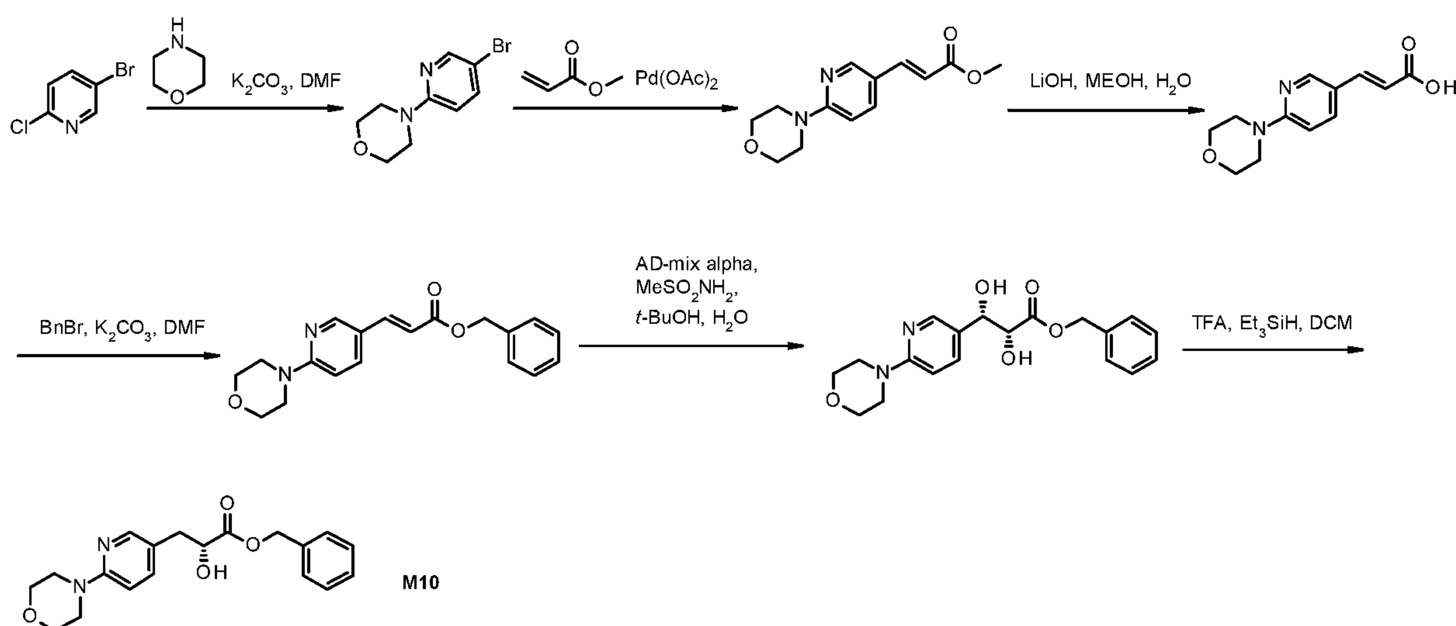
Scheme 8
