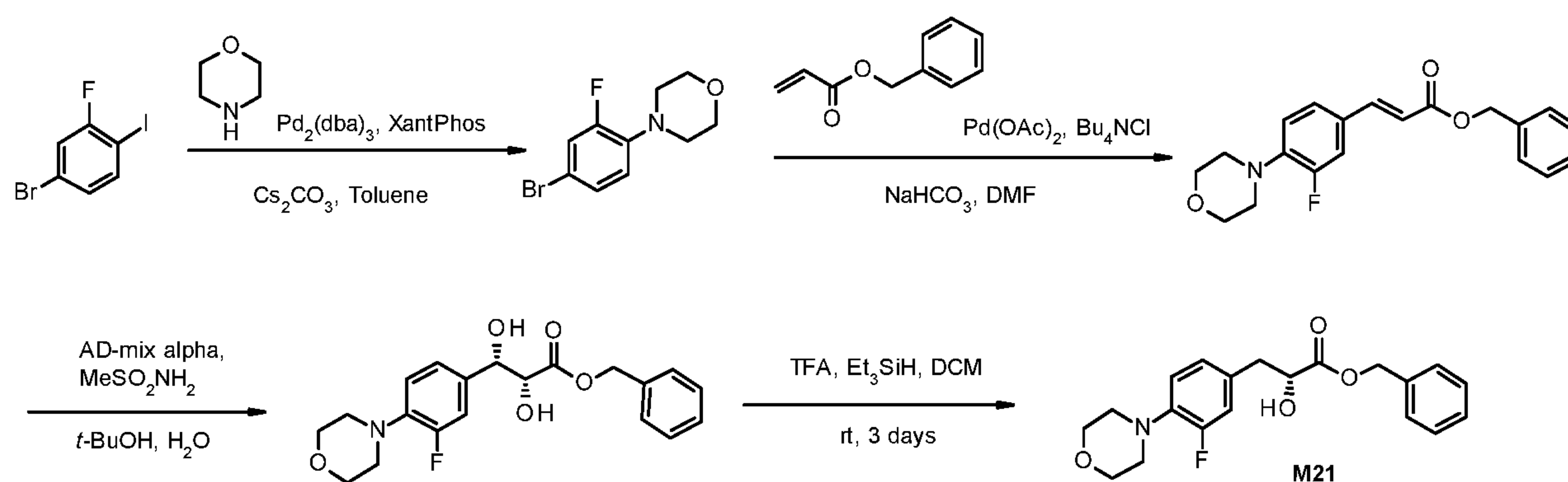
Scheme 14
