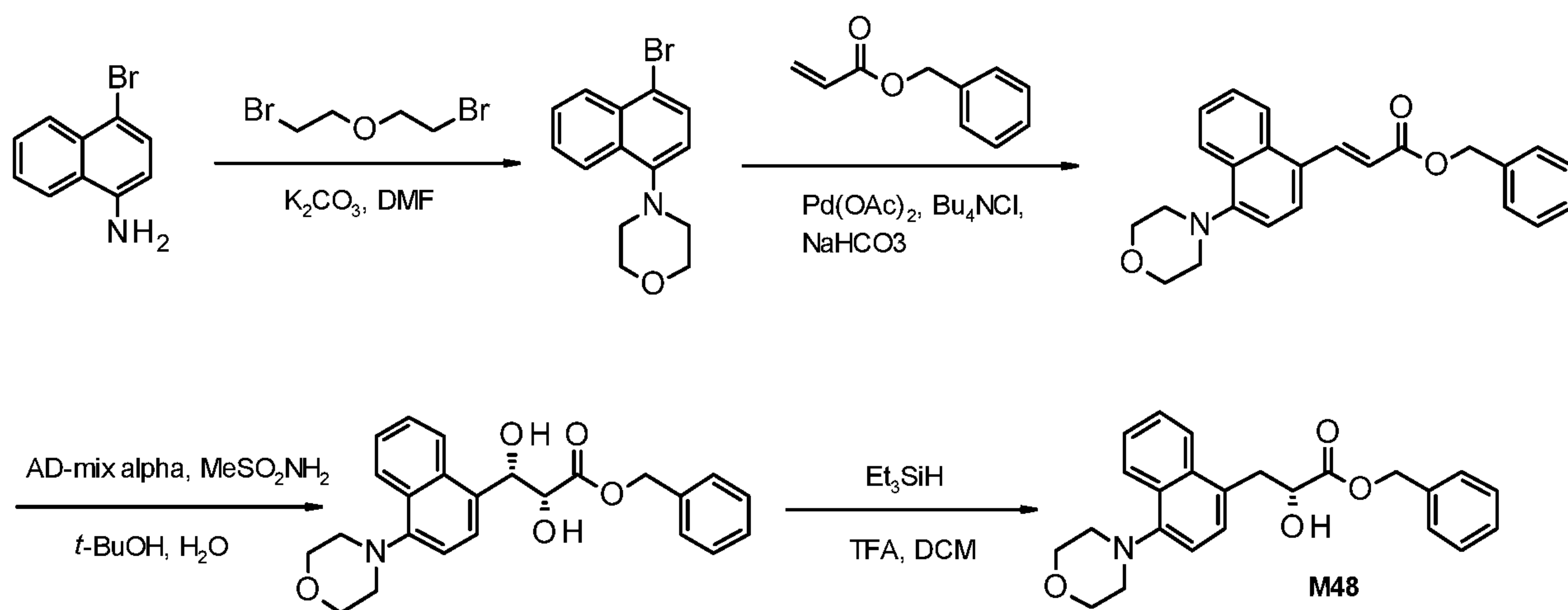
Scheme 26
