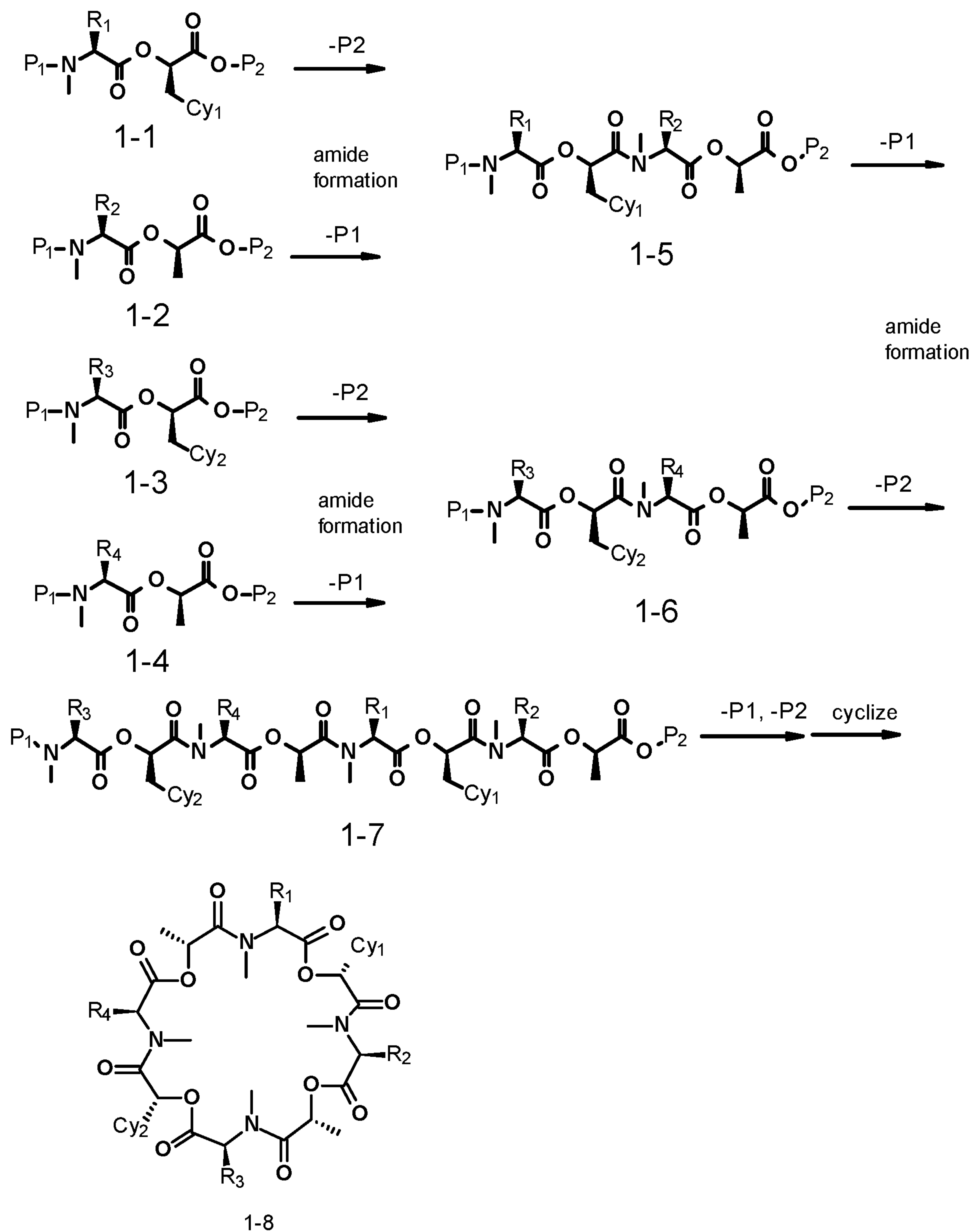
Scheme 1
