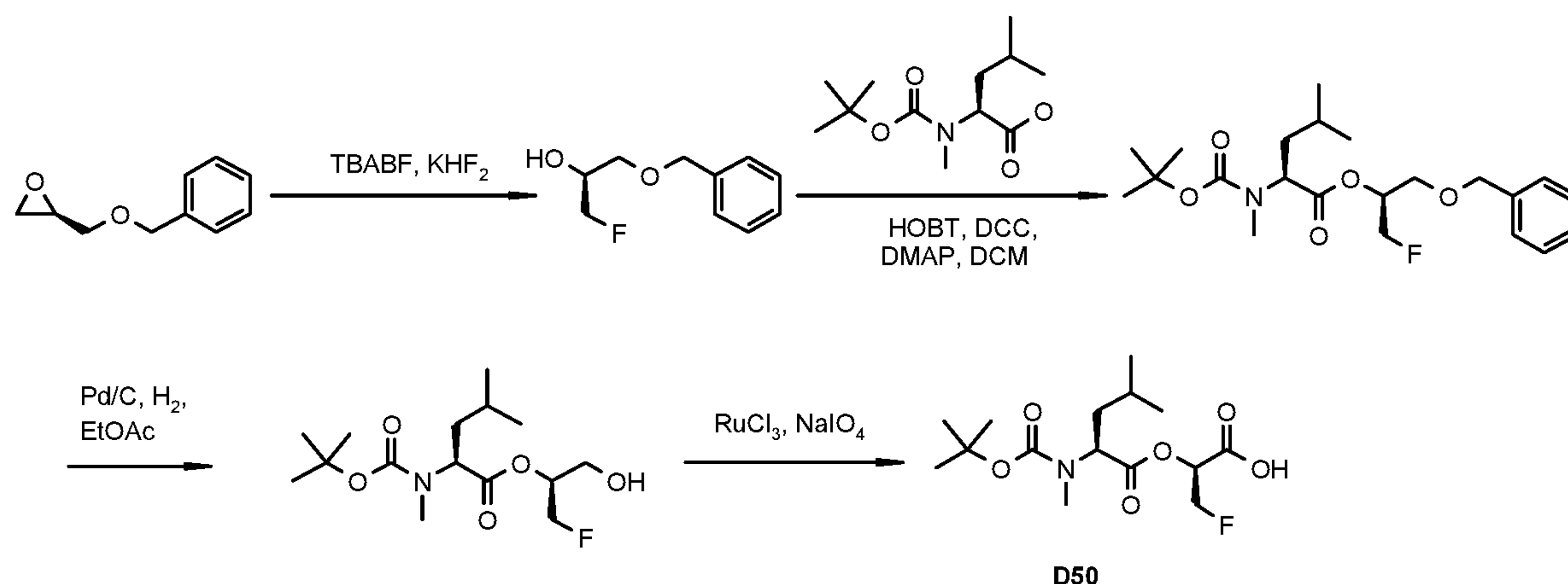
Scheme 29
