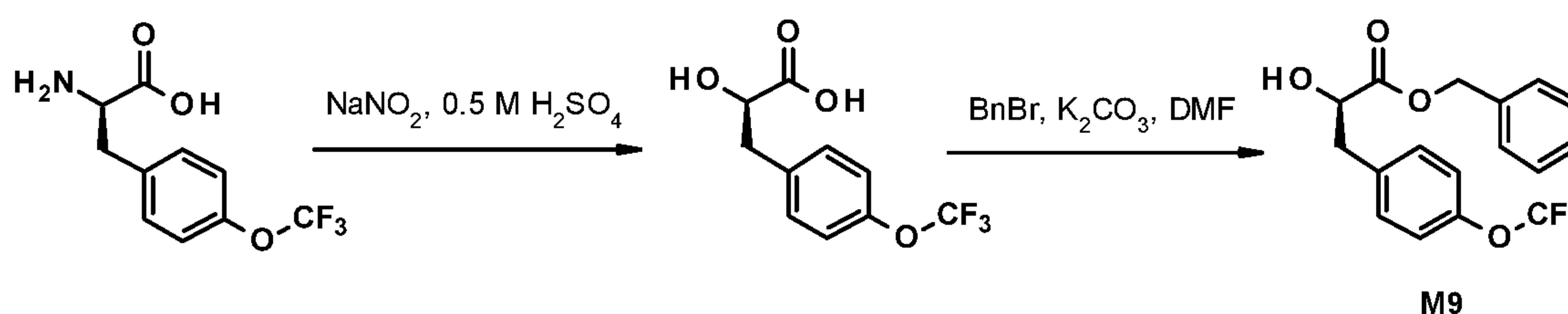
Scheme 7
