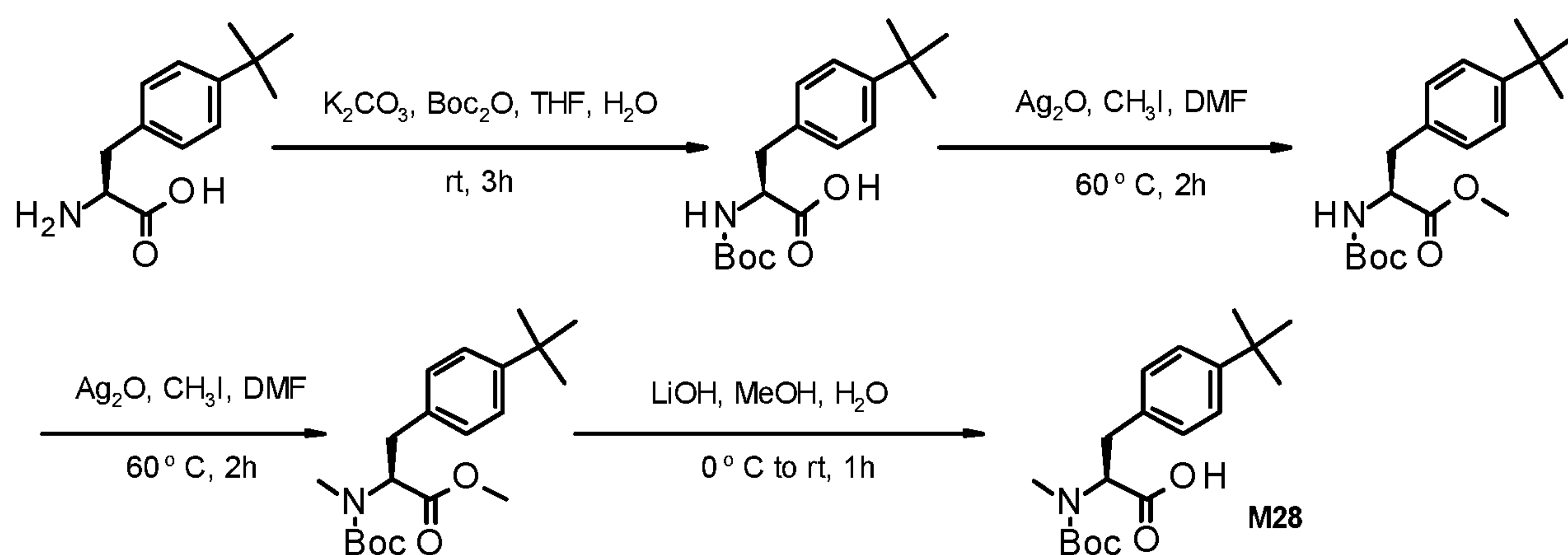
Scheme 17
