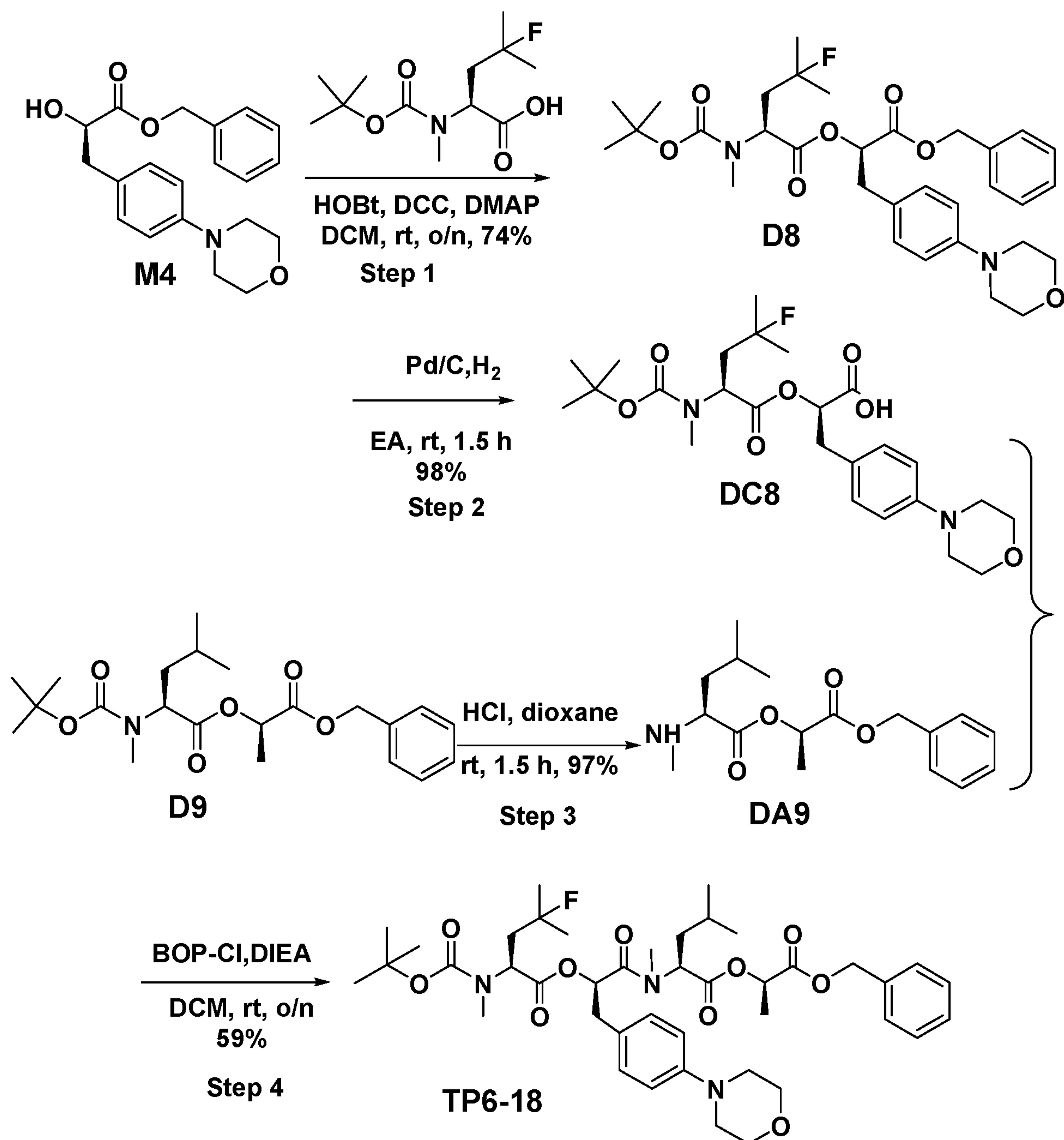
Scheme 34
