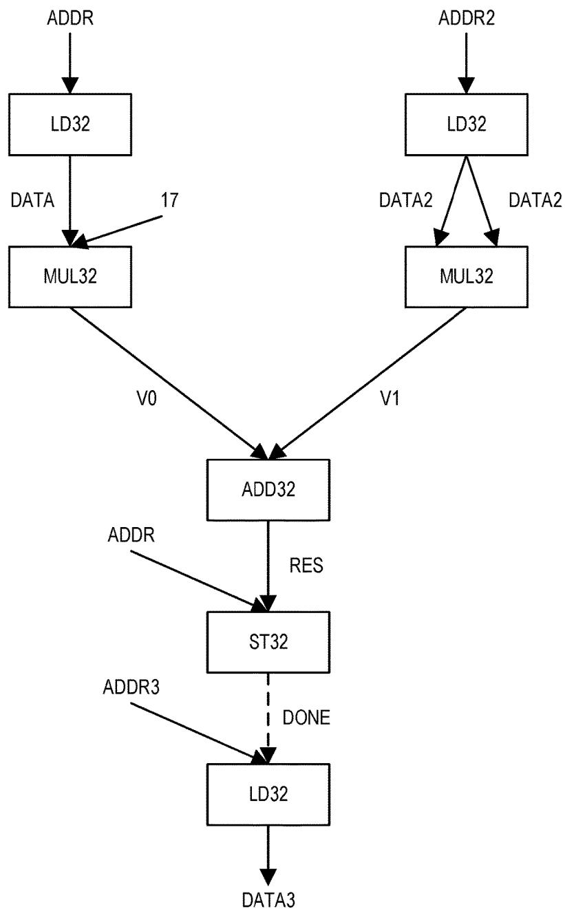
DATAFLOW GRAPH 3506
