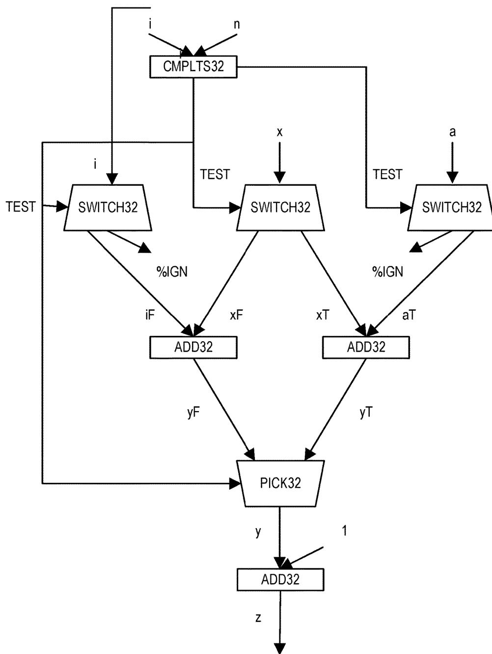
DATAFLOW GRAPH 3606
