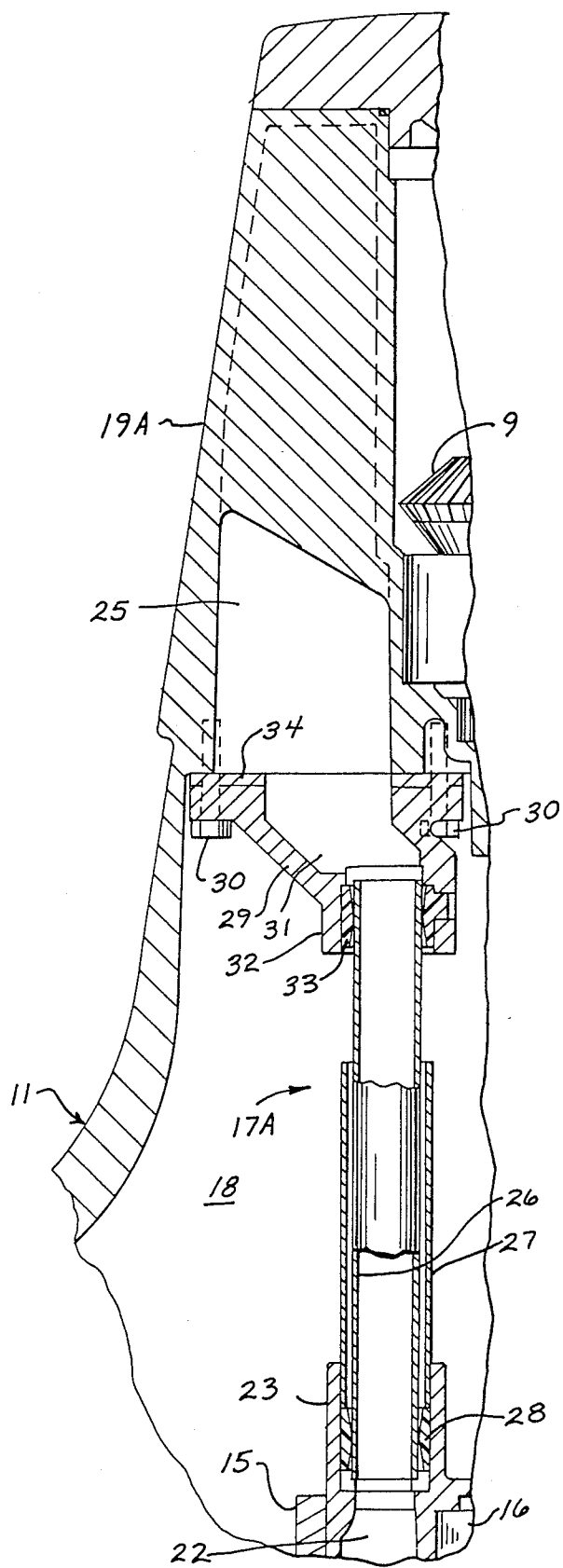
FIG. 3 PRIOR ART
