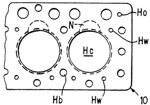
FIG. 2 (PRIOR ART)
