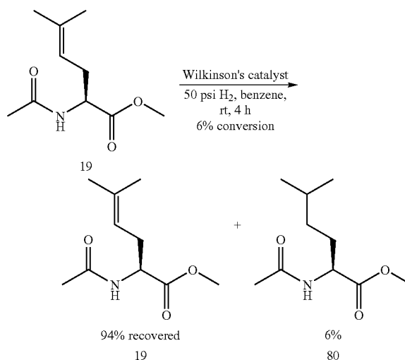
Scheme 4.31
