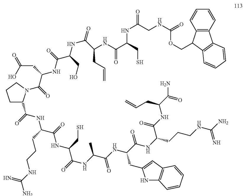
[2,8]-Cys-[3,12]-Hag conotoxin ImI: Fmoc-Gly-Cys-Hag-Ser-Asp-Pro-Arg-Cys-Ala-Trp-Arg-Hag-NH 2
