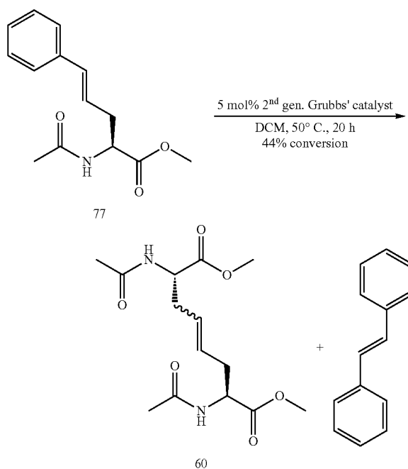
Scheme 4.26
