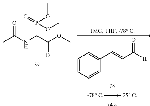
Scheme 4.23
