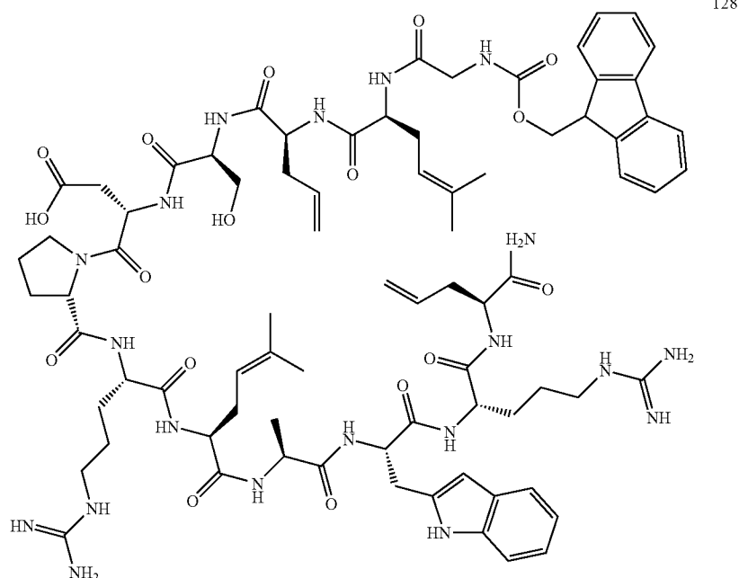
[2,8]-Pre-[3,12]-Hag conotoxin ImI: Fmoc-Gly-Pre-Hag-Ser-Asp-Pro-Arg-Pre-Ala-Trp-Arg-Hag-NH 2
