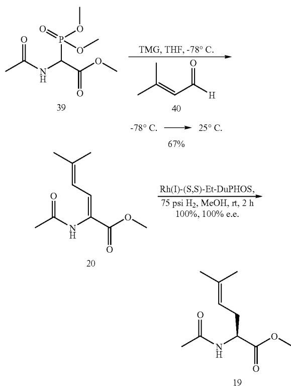
Scheme 4.30
