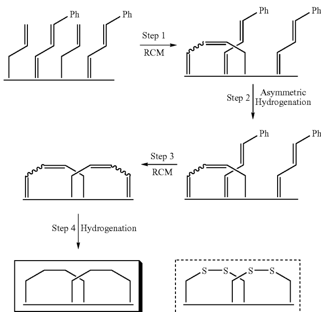
Scheme 4.22
