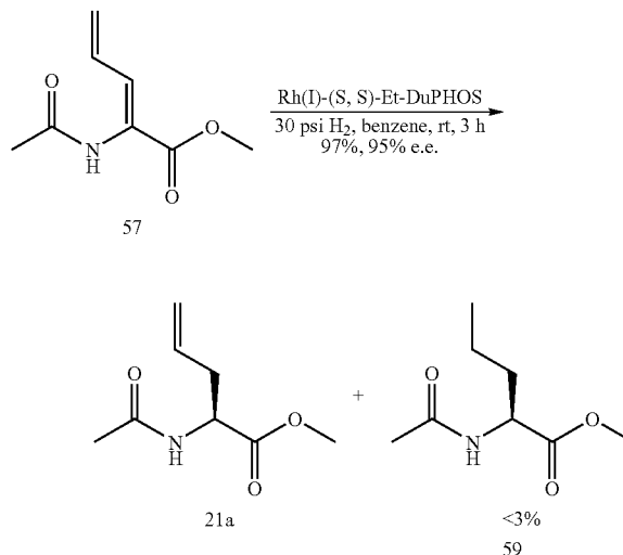
Scheme 4.5
