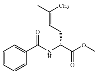
(2 R )-Methyl 2- N -benzoylamino-5-methylhex-4-enoate 87
