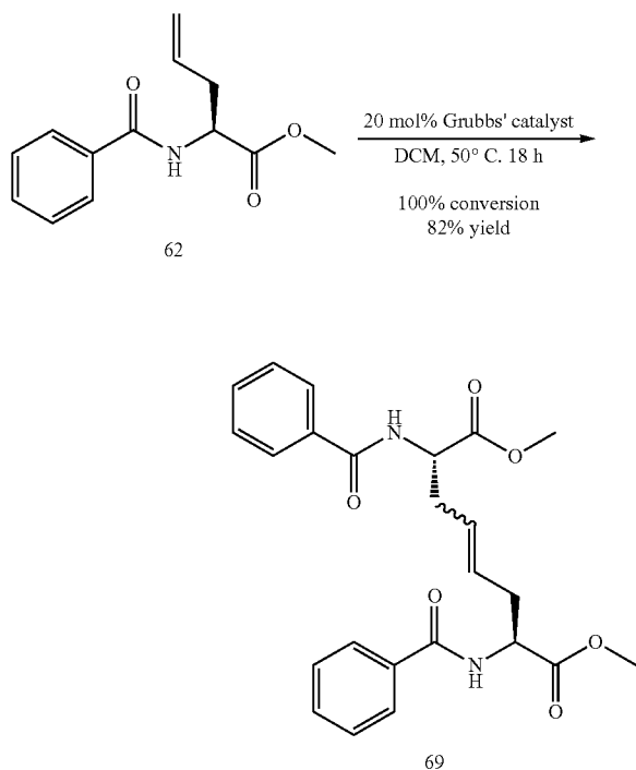
Scheme 4.17
