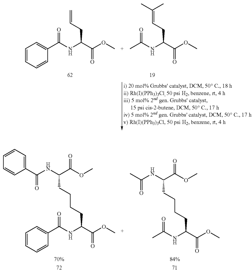
Scheme 4.35
