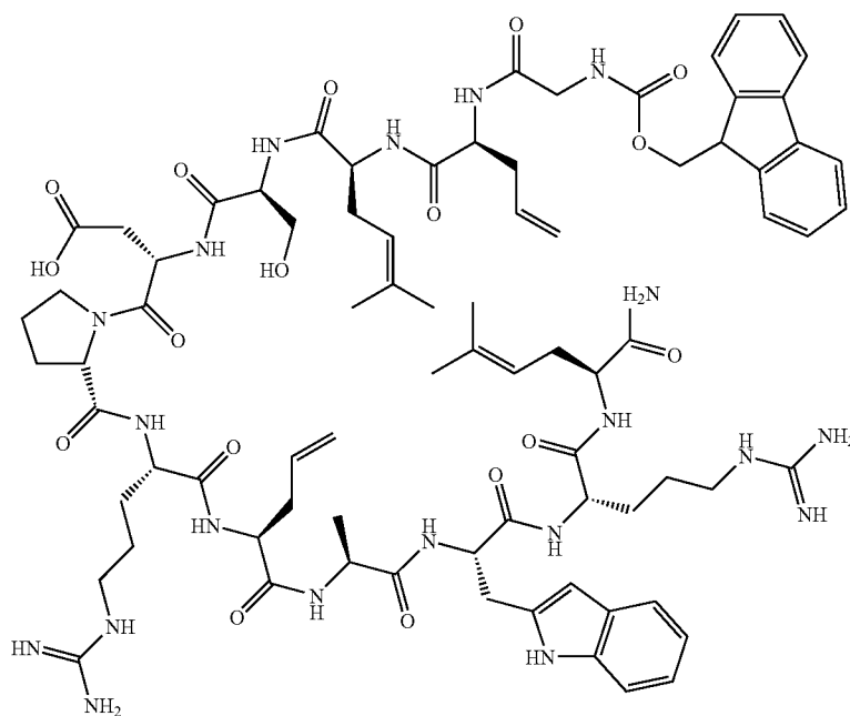
[2,8]-Hag-[3,12]-Pre conotoxin ImI: Fmoc-Gly-Hag-Pre-Ser-Asp-Pro-Arg-Hag-Ala-Trp-Arg-Pre-NH 2
