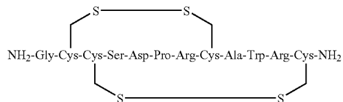
Native \alpha -Conotoxin ImI (Ctx)
