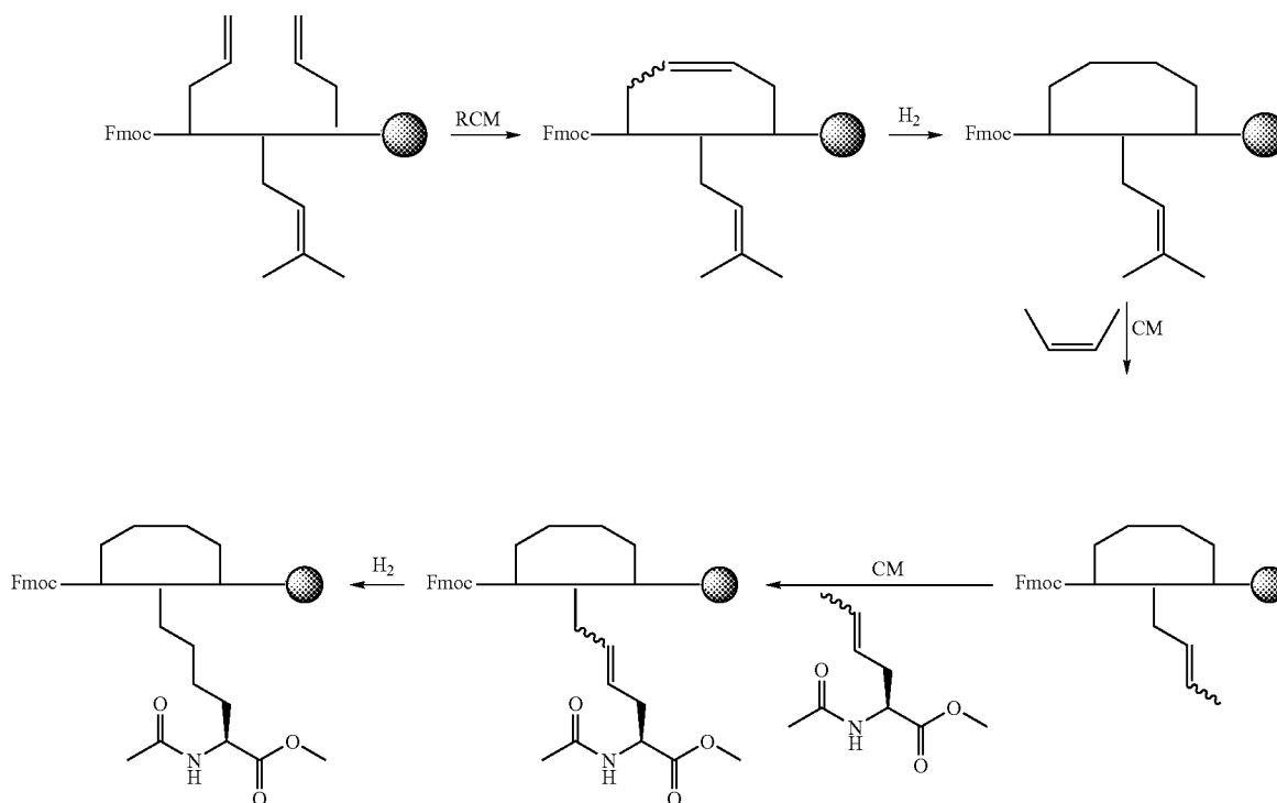
Scheme 6.7
