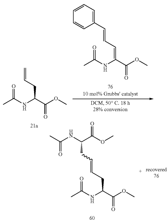
Scheme 4.24
