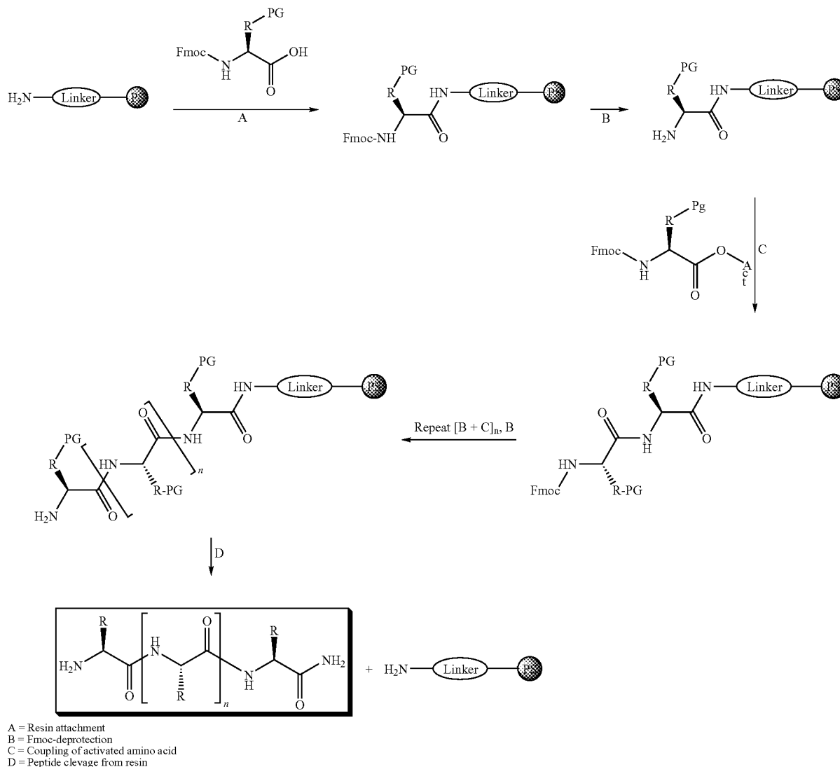
Scheme 6.1
