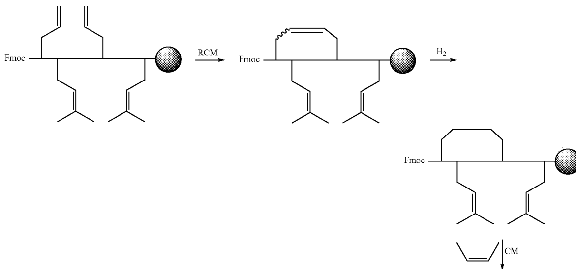
Scheme 6.21
