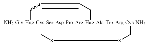
Dicarba-Cystino Ctx Hybrids
