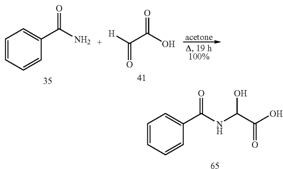
Scheme 4.12
