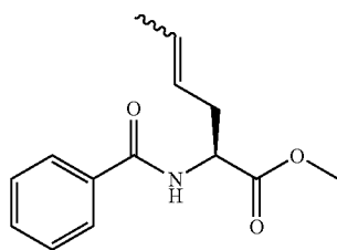
7.12.3 (2 S )-Methyl 2- N -Benzoylaminohex-4-enoate 88
