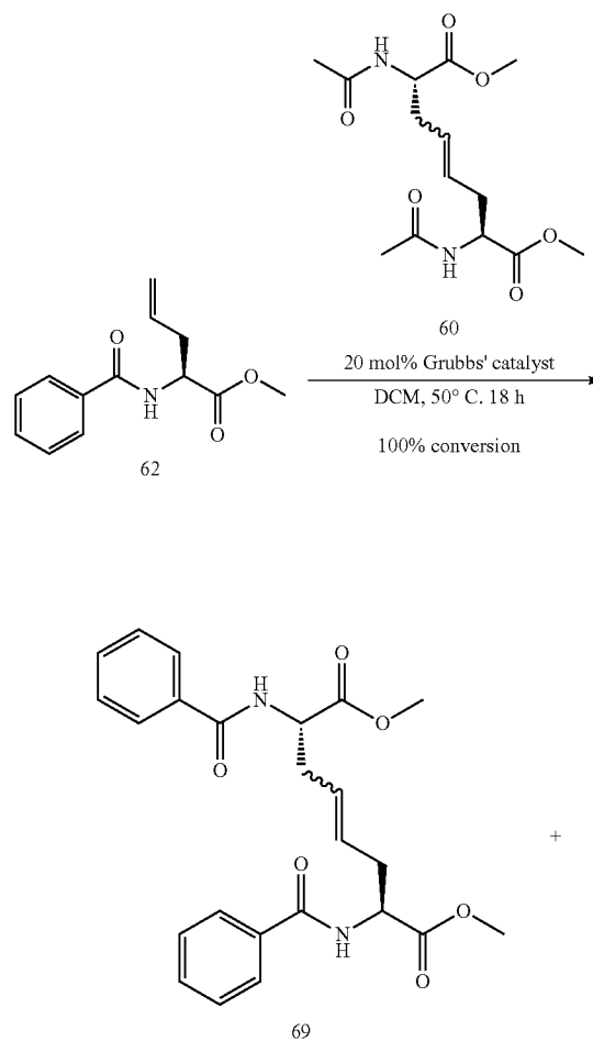
Scheme 4.18
