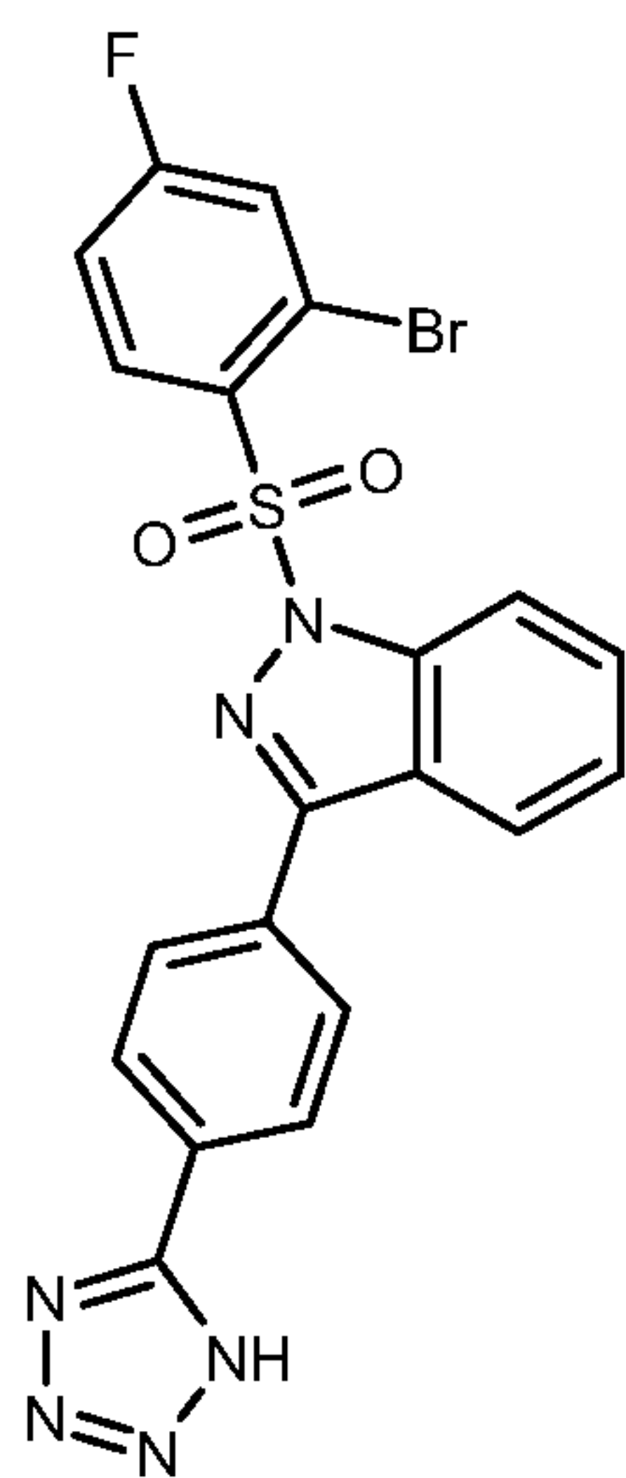
21B: 3-(4-(1H-tetrazol-5-yl)phenyl)-1-(2-bromo-4-fluorophenylsulfonyl)-1H-indazole
