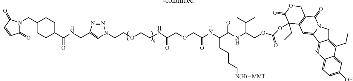
Precursor of CL7-SN-38
