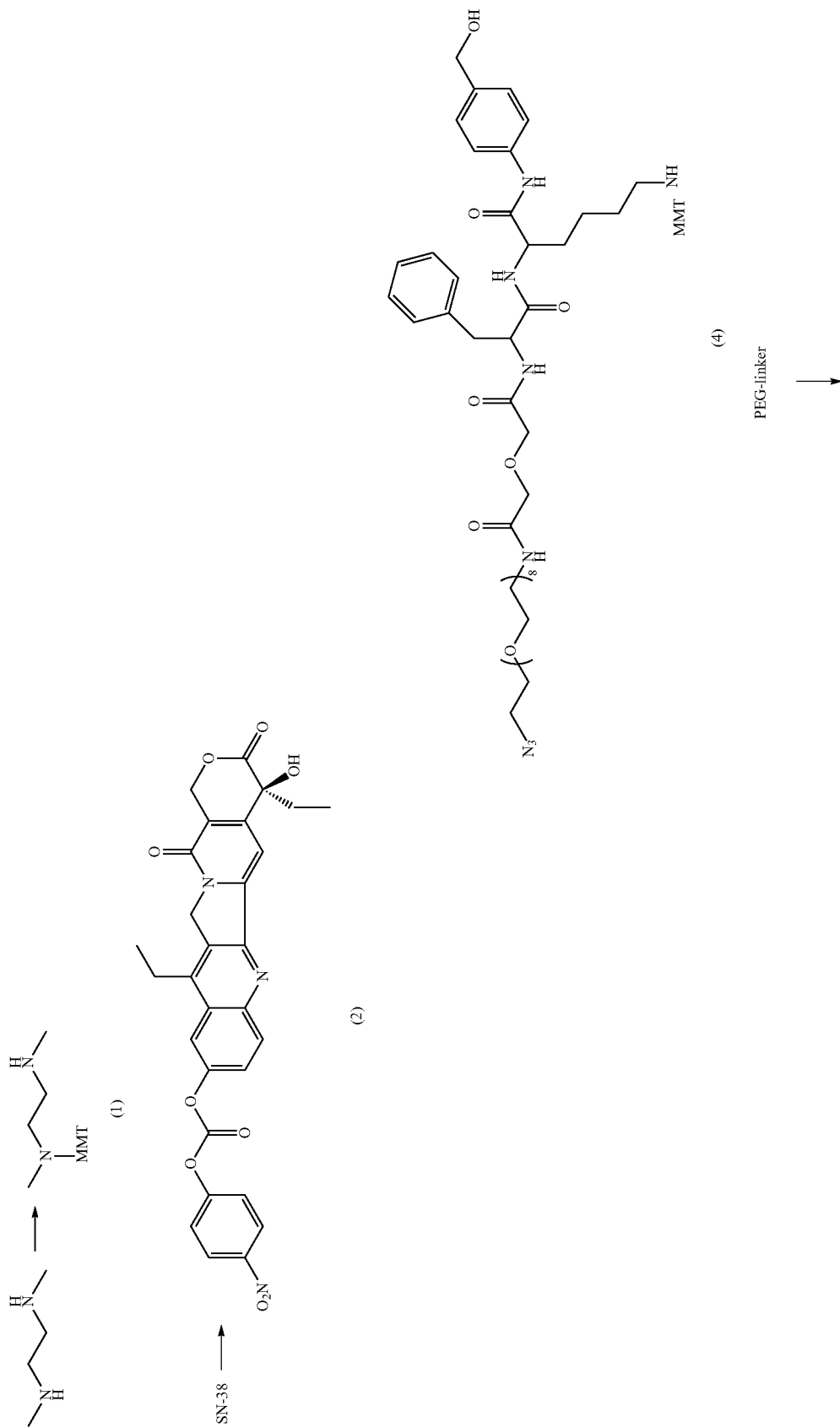
Scheme-4: Preparation of CL2E-SN-38
