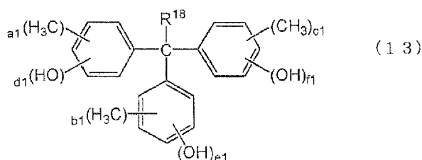
[Chemical Formula 8]
