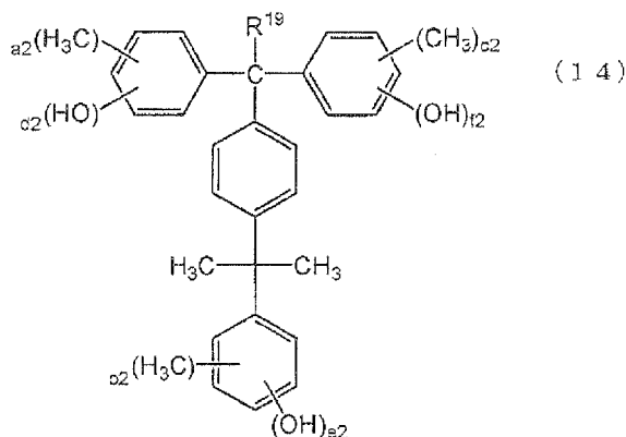
[Chemical Formula 9]
