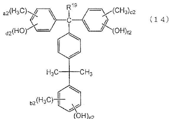
[Chemical Formula 22]
