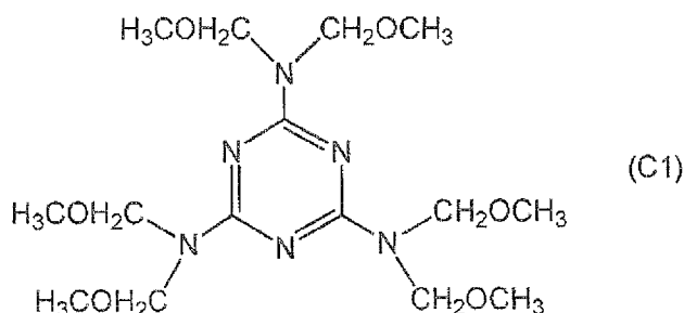
[Chemical Formula 24]
