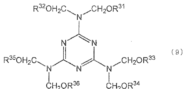
[Chemical Formula 15]
