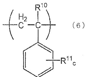
[Chemical Formula 12]
