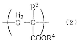
[Chemical Formula 16]
