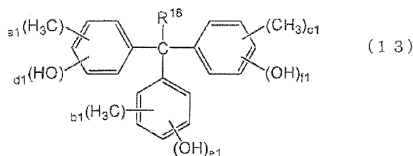
[Chemical Formula 21]
