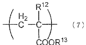
[Chemical Formula 7]
