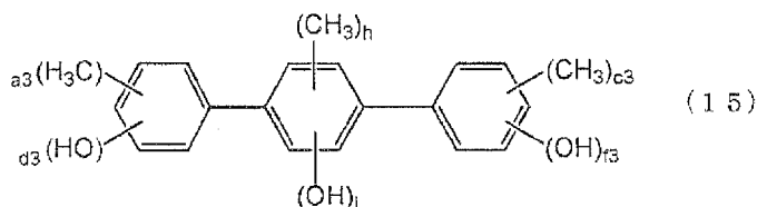
[Chemical Formula 10]
