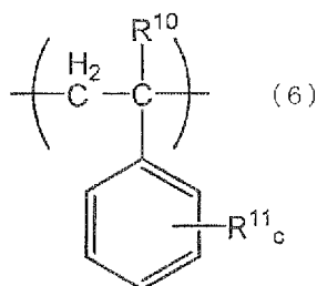
[Chemical Formula 6]
