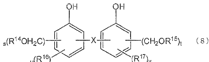
[Chemical Formula 14]
