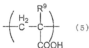
[Chemical Formula 5]
